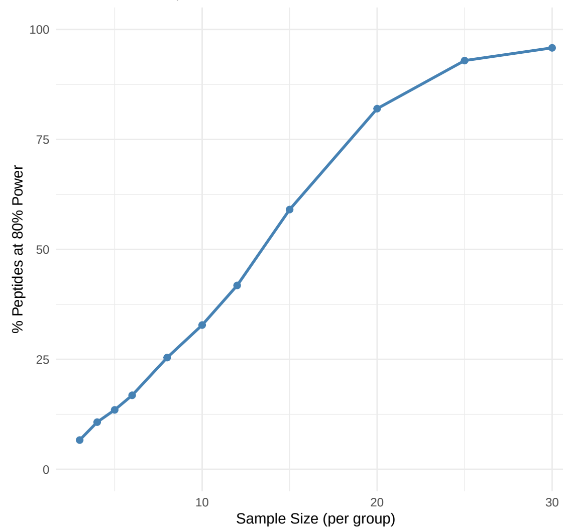
E Q2: Sample Size for 80% Power
