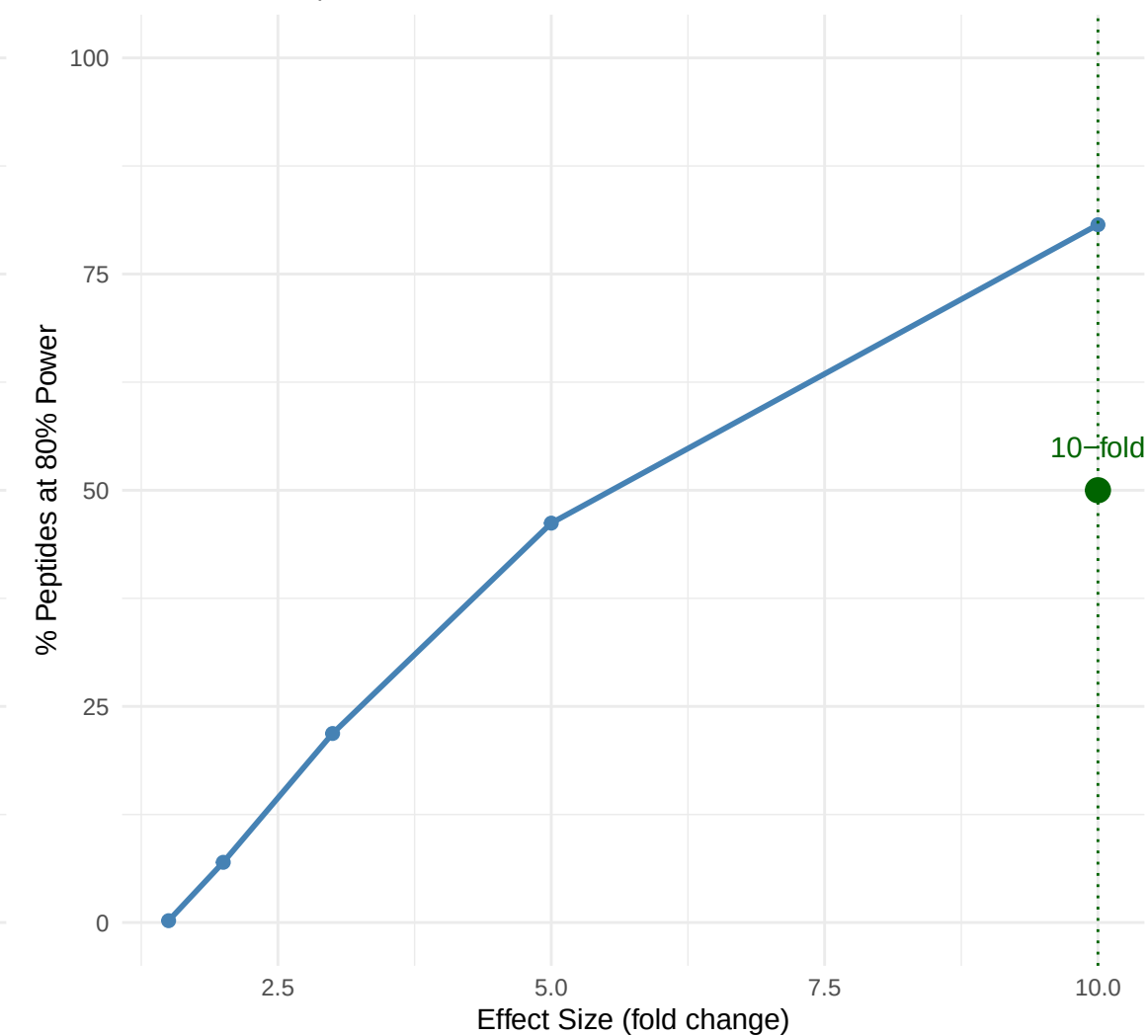
F Q3: Minimum Detectable Effect
