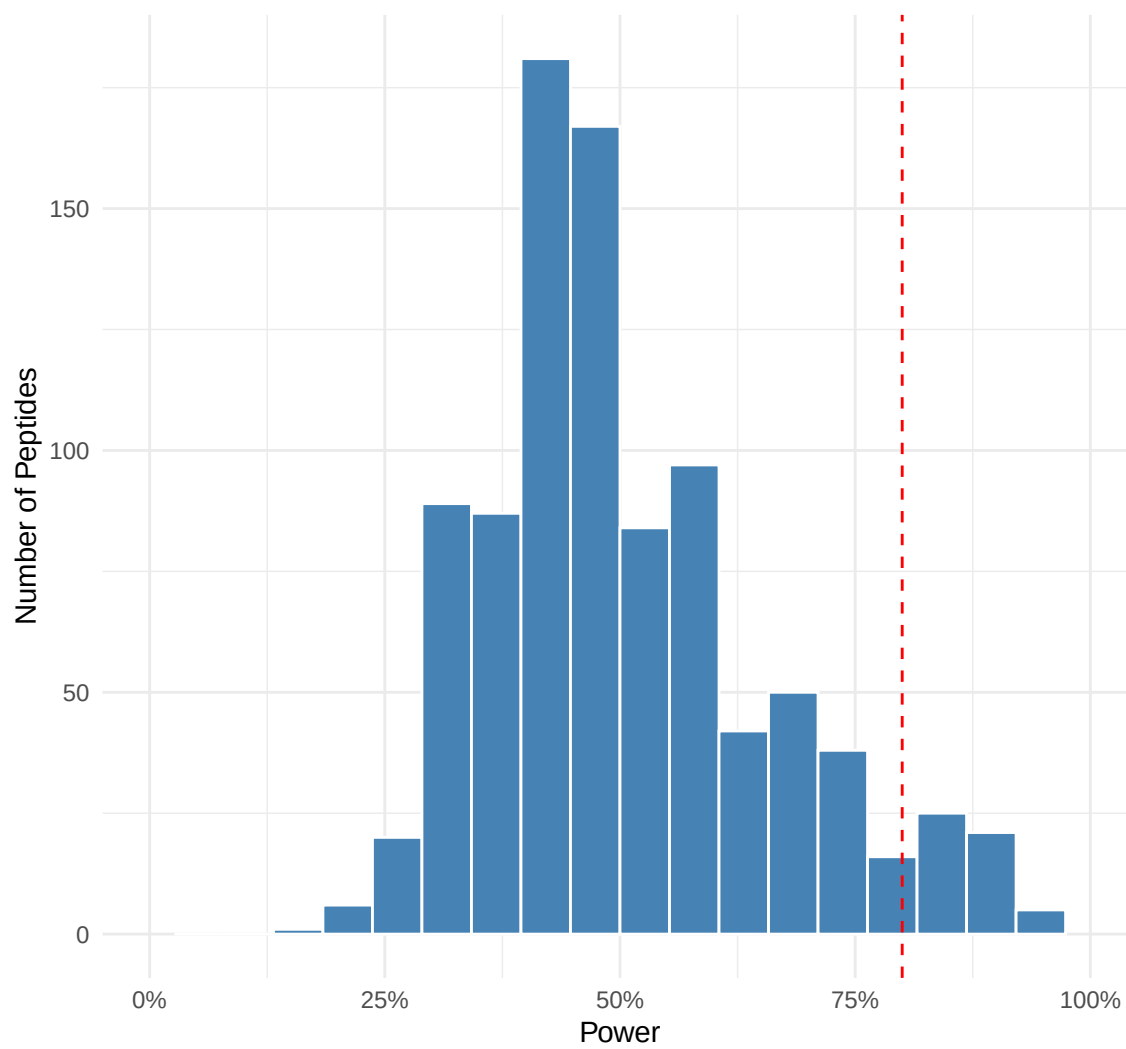
D Q1: Current Power (N=3, 2-fold)
