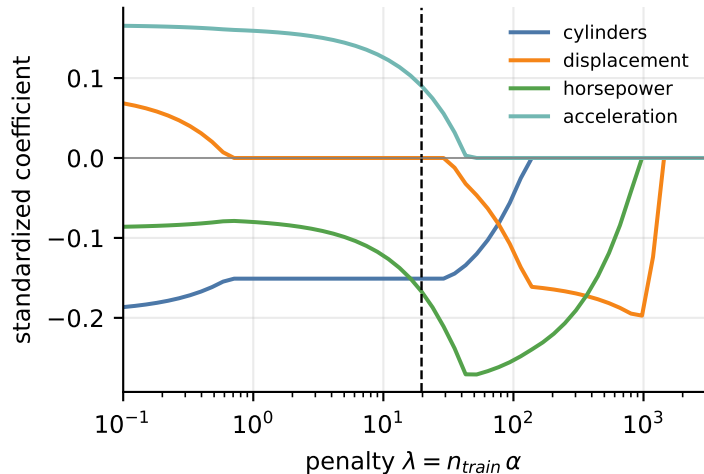
Lasso, small predictors - statsmodels
