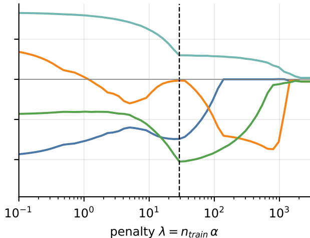
Lasso, small predictors - ScalaTion
