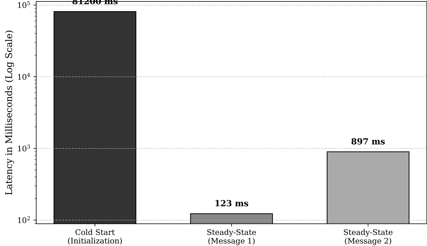
ZeroChat: Initialization Overhead vs. Steady-State Messaging Latency
