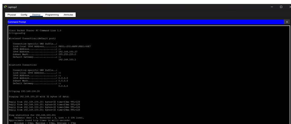
Figure 17: Successful Intra-VLAN Ping (Wireless Clients)
