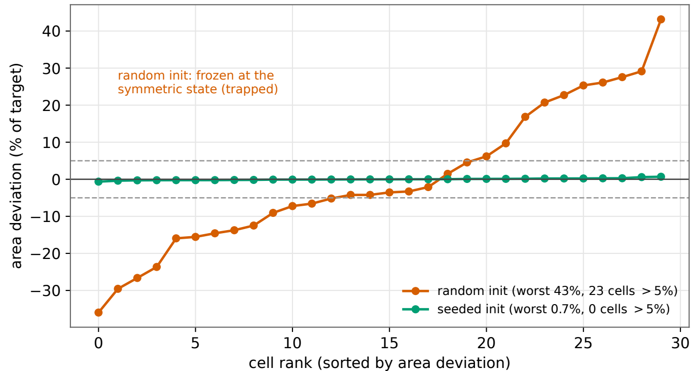
Corrected (steeper) energy: random init traps, seeded init escapes (N=30, \lambda=2.1 )
