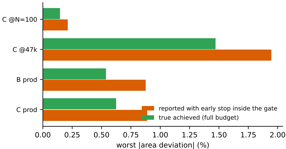
Early stopping inside the measurement path masked quality
