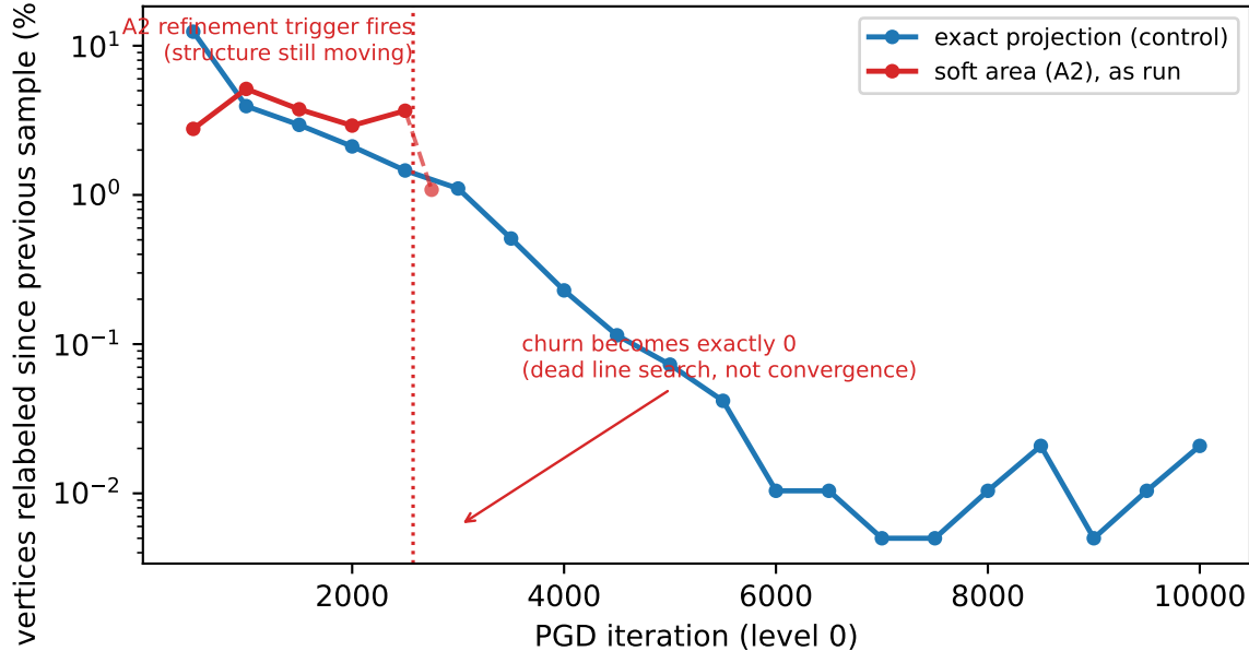
label churn from the identical seeded x_0 (stride 500)
