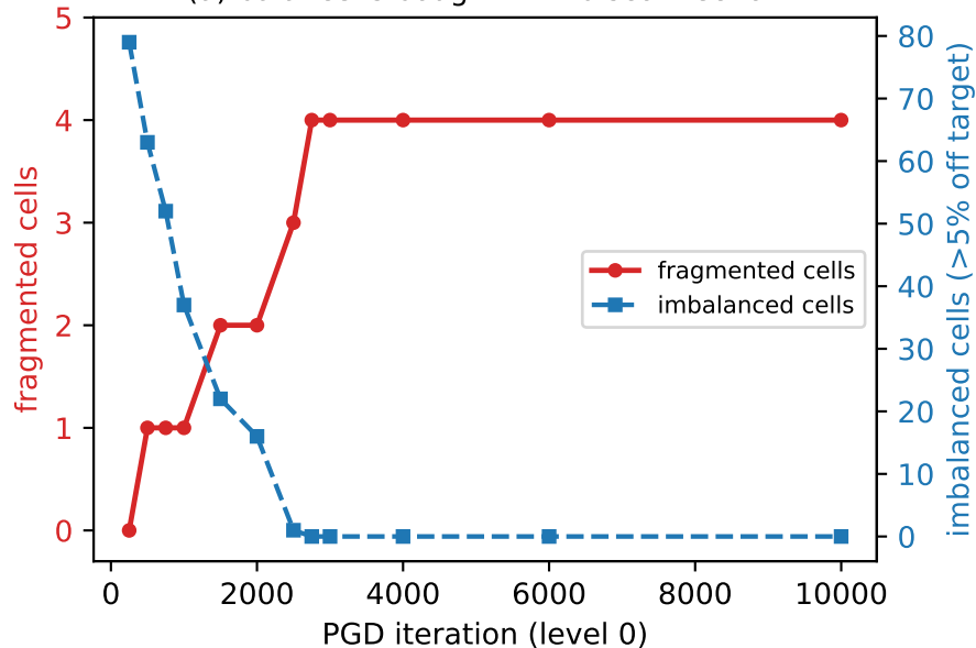
(a) balance is bought with disconnection
