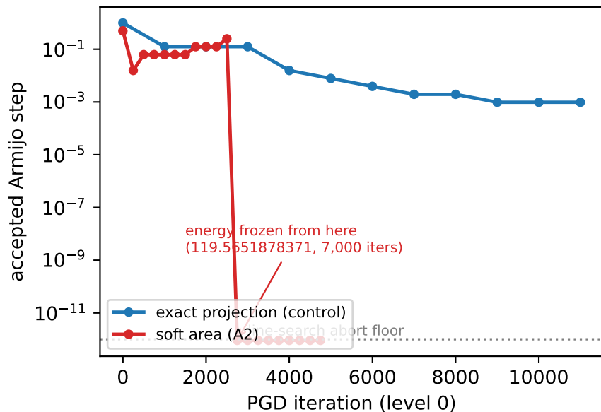
(b) the line search collapses
