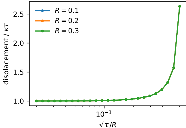
One-step displacement, exact
