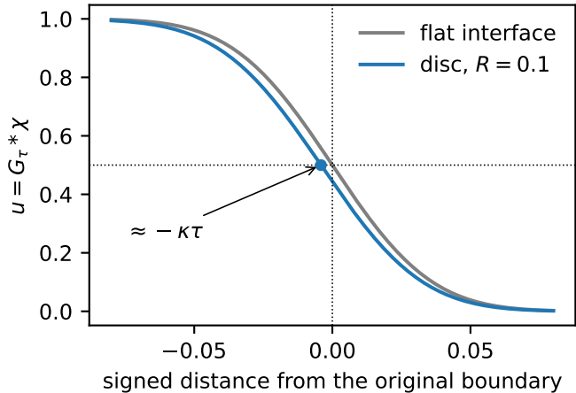
Diffused indicator, \sqrt{\tau} = 0.02
