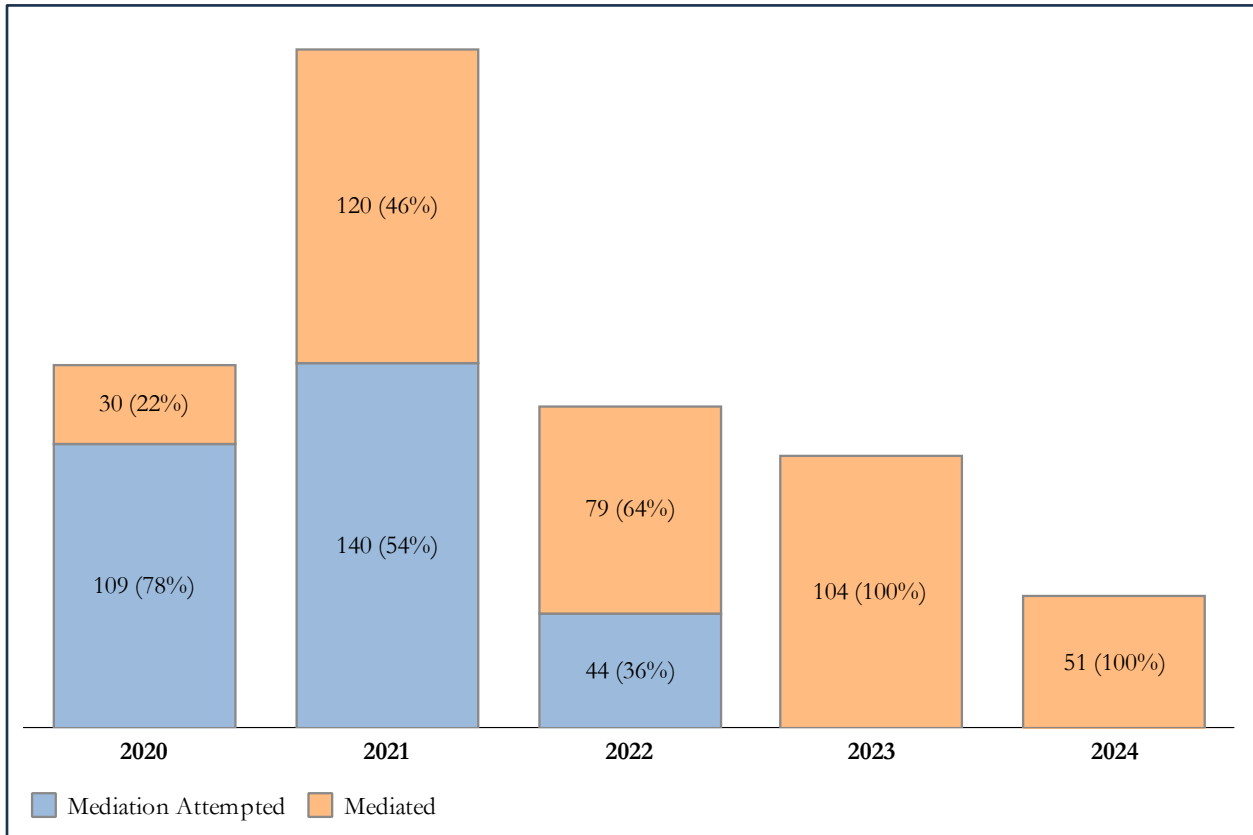
Figure 45: Mediation Closures
