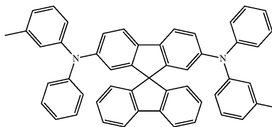
Spiro-TPD
