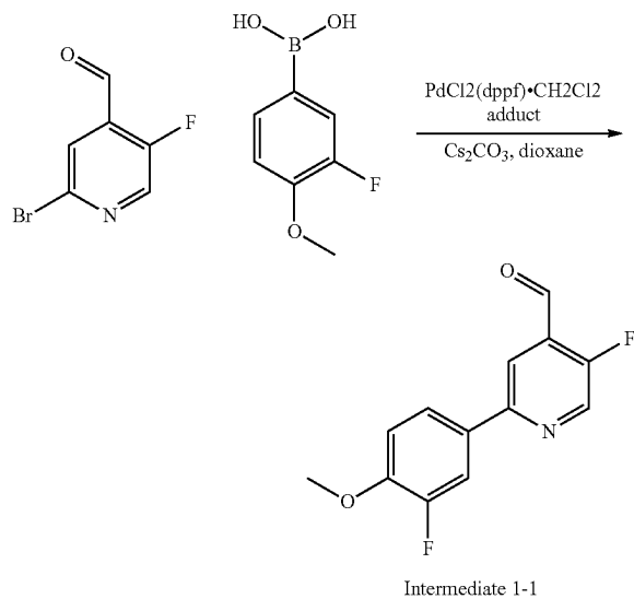
Intermediate 1-1: 5-Fluoro-2-(3-fluoro-4-methoxyphenyl)isonicotinaldehyde
