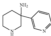
Intermediate 271-7: 3-(pyridin-3-yl)piperidin-3-amine
