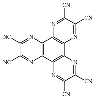
Hexanitrile hexaazatriphenylene
