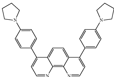
PrdP2Phen (101)
