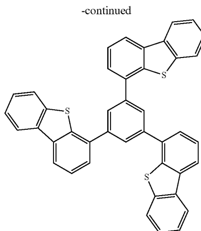
DBT3P-II
