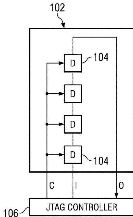
FIG. 1 (PRIOR ART)
