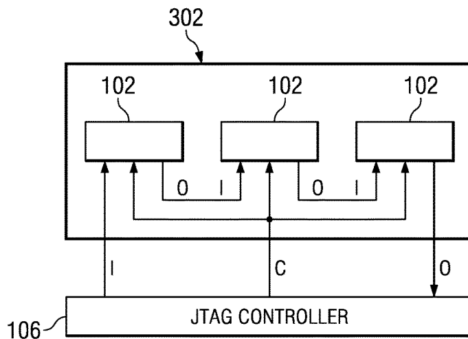
FIG. 3 (PRIOR ART)
