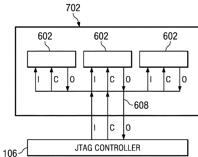
FIG. 7 (PRIOR ART)
