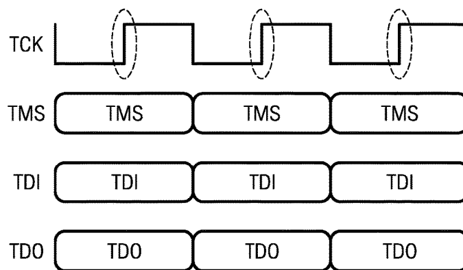
FIG. 5 (PRIOR ART)
