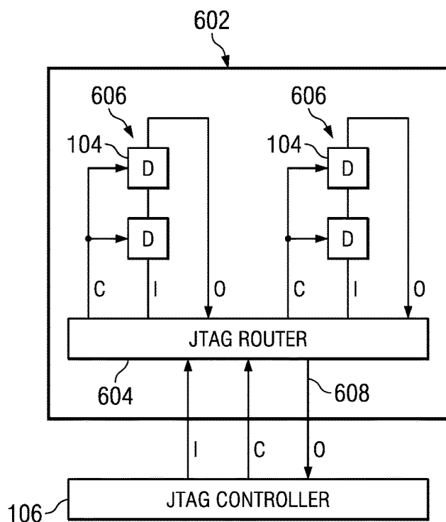
FIG. 6 (PRIOR ART)
