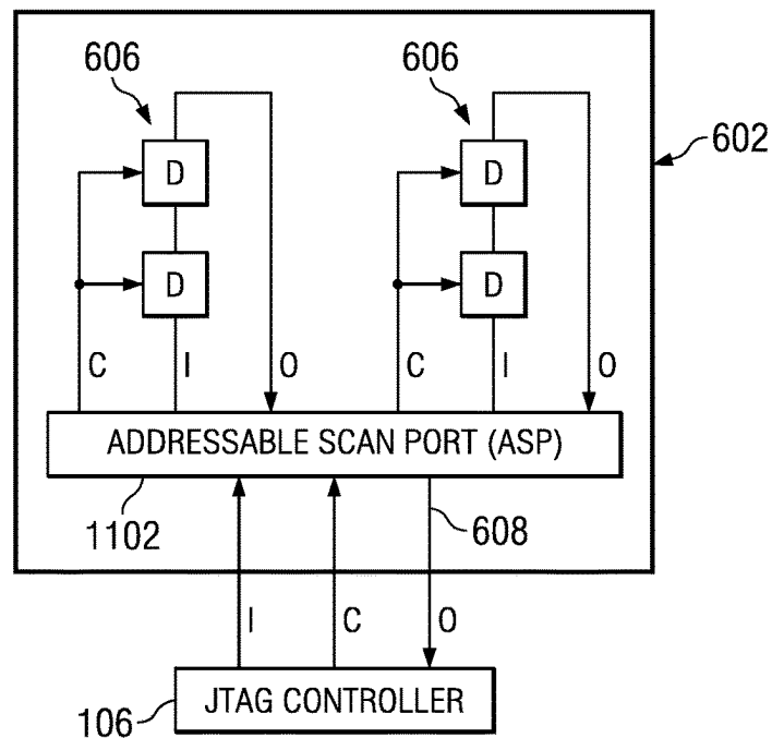
FIG. 11 (PRIOR ART)
