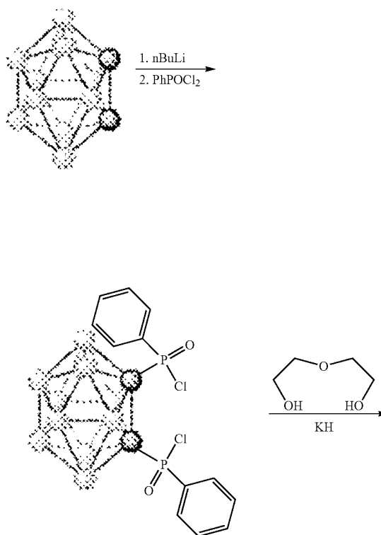
Scheme 1. Reaction scheme for phosphine oxide spacer carborane 9-crown-3 and proposed lithium capture/release mechanism
