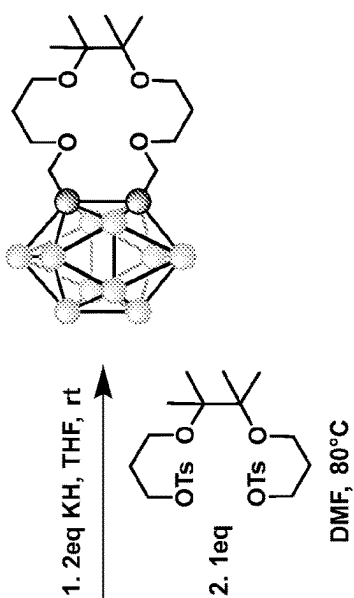
Cb 16-crown-4
