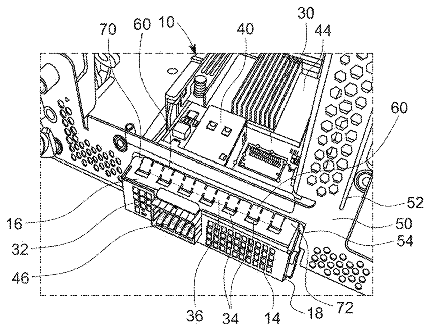
FIG. 1C (PRIOR ART)
