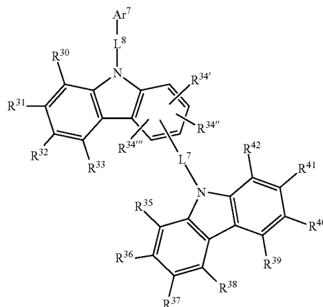
[Chemical Formula 2]
