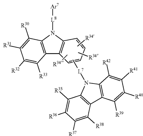
[Chemical Formula 2]
