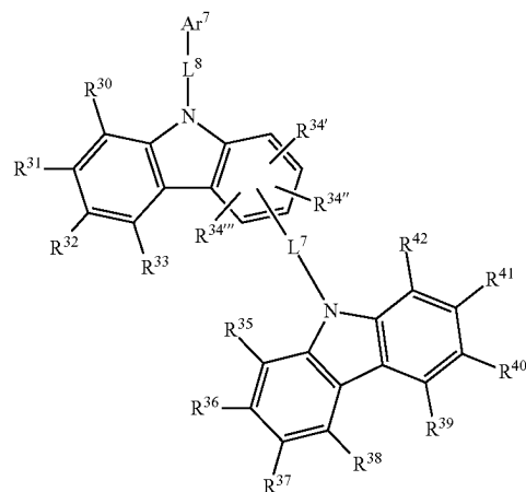
[Chemical Formula 2]
