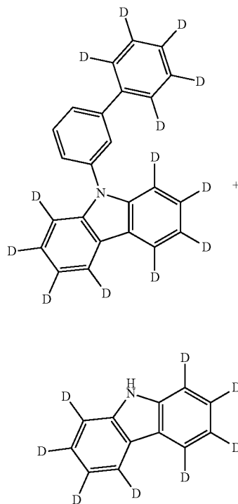
[Reaction Scheme 2]
