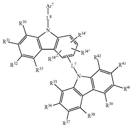
[Chemical Formula 2]
