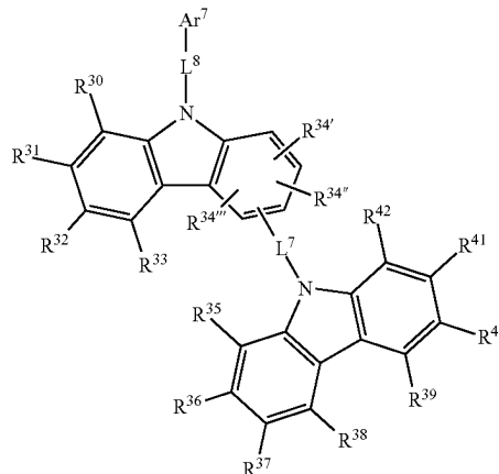
[Chemical Formula 2]
