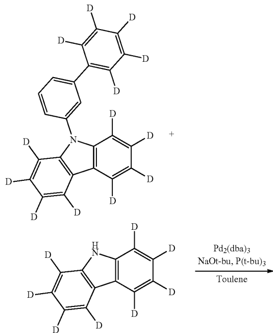
[Reaction Scheme 2]
