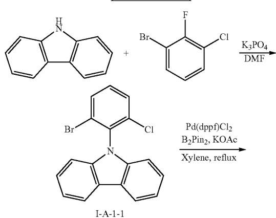
[Reaction Scheme 1]
