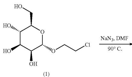
Compound 3: 1-(2-aminoethyl)- \alpha -D-mannose
