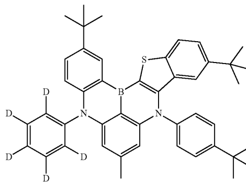
DF8(DABNA-1)
