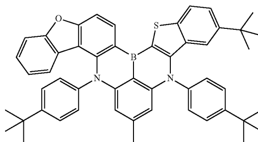
DF11
