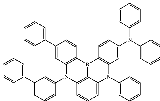
DF9(DABNA-2)
