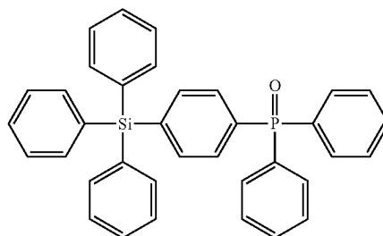
TSP01
