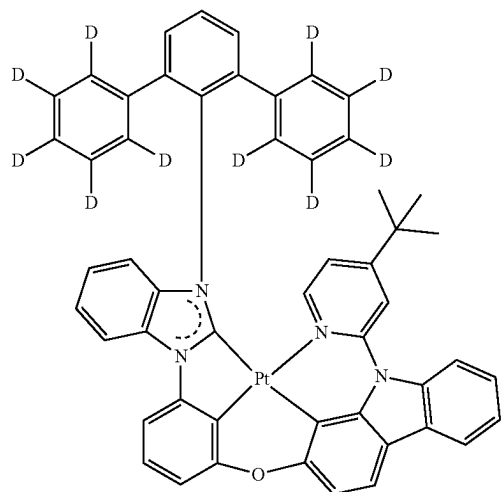
PD39
