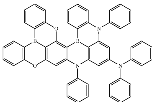
DF13
