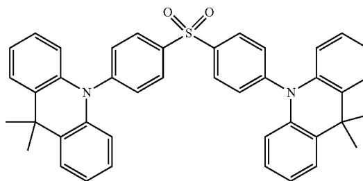
(DMAC-DPS)
