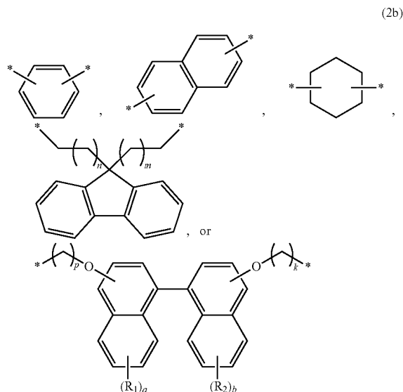
[Chemical Formula 4]
