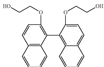
BNE 2,2'-bis(2-hydroxyethoxy)-1,1'-binaphthalene
