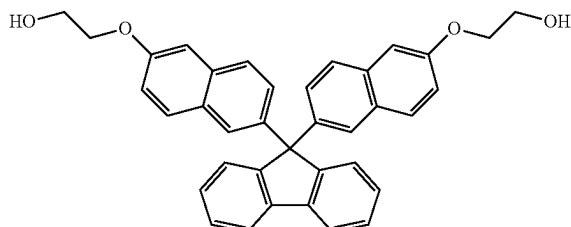
BNEF 9,9-bis(6-(2-hydroxyethoxy)naphthalene-2-yl)fluorene
