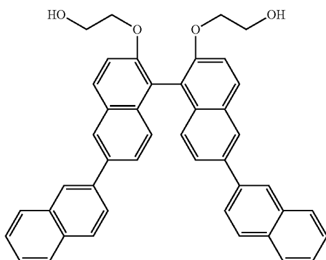
2DNBINOL-2EO 2,2'-bis(2-hydroxyethoxy)-6,6'-di(phenanthrene-9-yl)- 1,1'-binaphthalene
