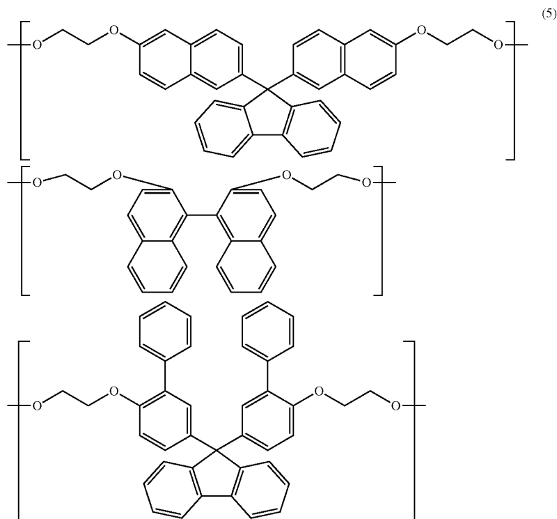
[Chemical Formula 17]
