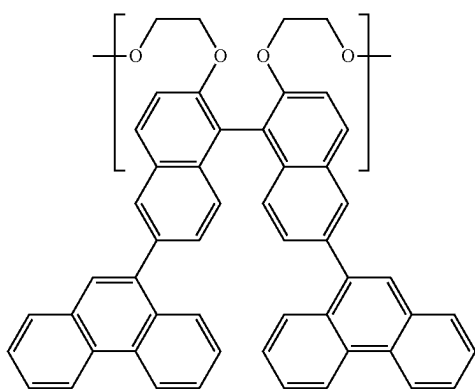
[Chemical Formula 27]
