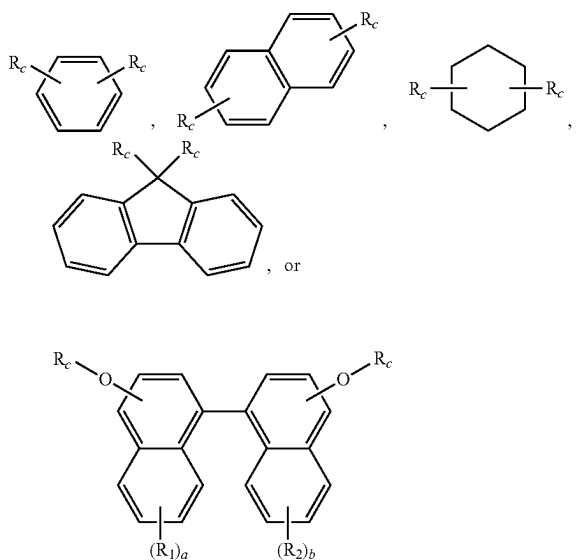
[Chemical Formula 5]
