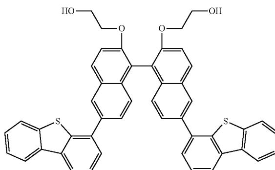
THI-BNA 6,6'-di-(dibenzo[b,d]thiophene-4-yl)-2,2'-bis-(2- hydroxyethoxy)-1,1'-binaphthalene
