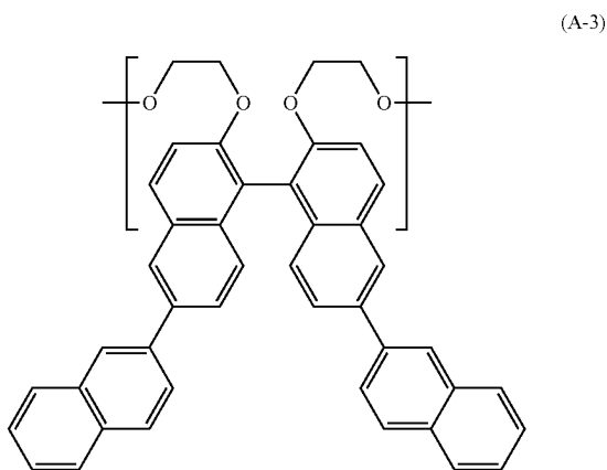
[Chemical Formula 8]
