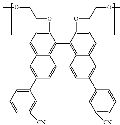
[Chemical Formula 29]
