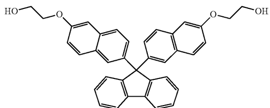
BNEF 9,9-bis(6-(2-hydroxyethoxy)naphthalene-2-yl)fluorene
