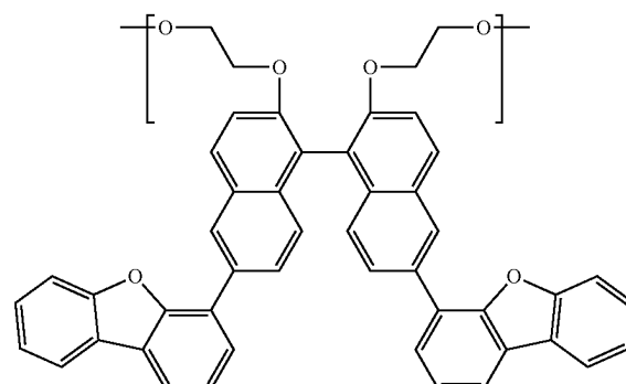
[Chemical Formula 30]
