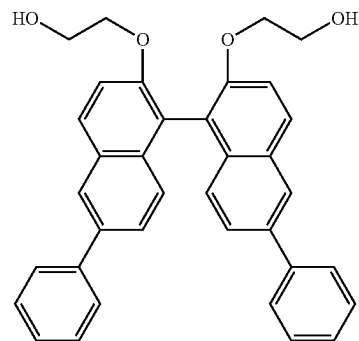
(BINL-2EO or 6,6'-DPBHBNA)
