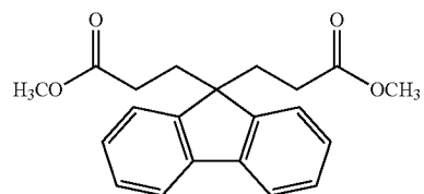
FDPM 9,9-fluorene-methyl dipropionate
