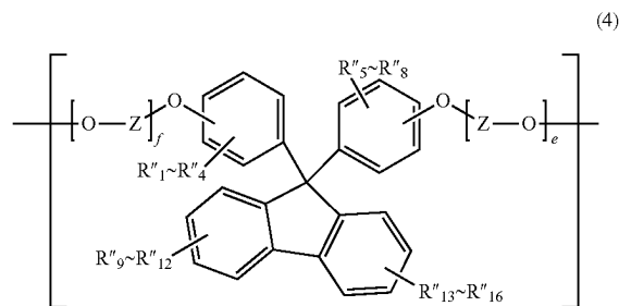
[Chemical Formula 32]
