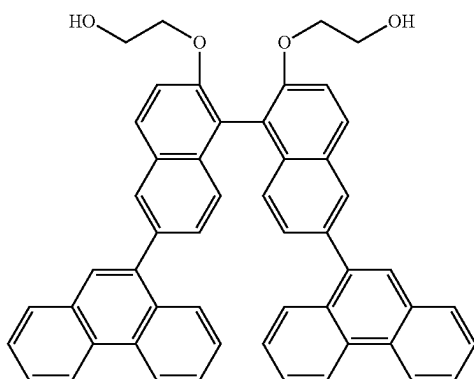
9DPNBINOL-2EO 2,2'-bis(2-hydroxyethoxy)-6,6'-di(phenanthrene-9-yl)- 1,1'-binaphthalene
