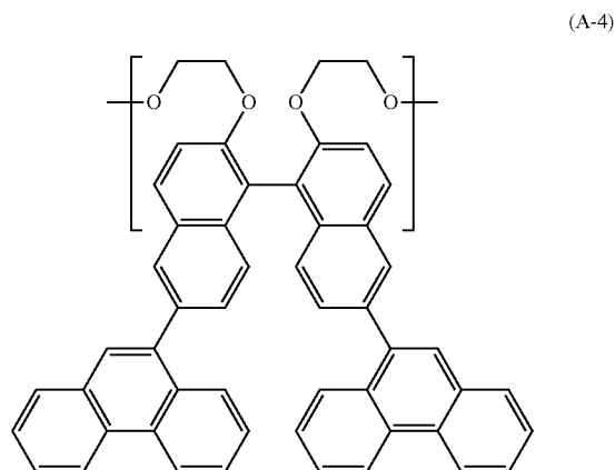
[Chemical Formula 9]
