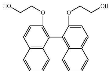
BNE 2,2'-bis-(2-hydroxyethoxy)-1,1'-binaphthalene
