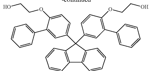
BPPEF 9,9-bis(4-(2-hydroxyethoxy)-3-phenylphenyl)fluorene
