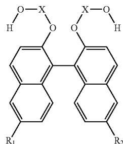
[Chemical Formula 36]
