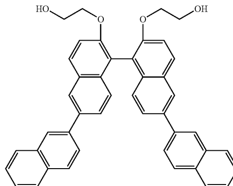
(2DN BINOL-2EO)
