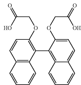
BINOL-DC 2,2'-bis(2- hydroxycarbonylmethoxy)- 1,1'-binaphthyl
