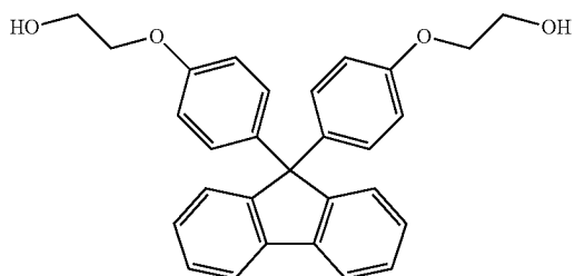
BPPEF 9,9-bis[4-(2-hydroxyethoxy)phenyl]fluorene
