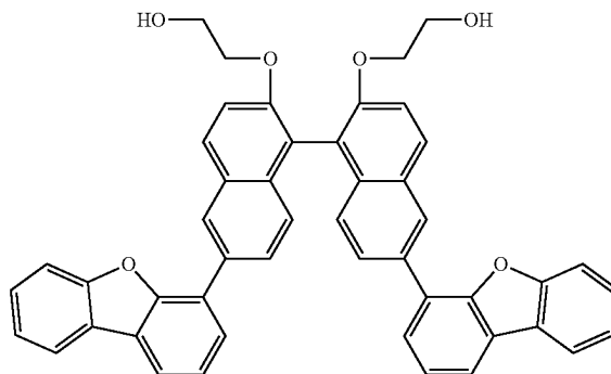
FUR-BNA 6,6'-di-(dibenzo[b,d]furan-4-yl)-2,2'-bis-(2- hydroxyethoxy)-1,1'-binaphthalene
