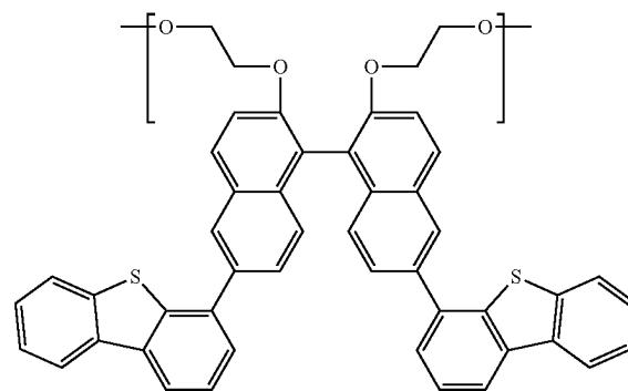
[Chemical Formula 30]
