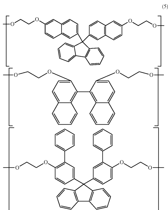
[Chemical Formula 33]
