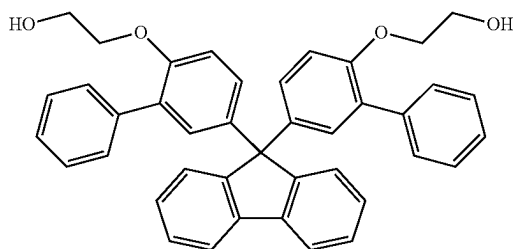
BPPEF 9,9-bis(4-(2-hydroxyethoxy)-3-phenylphenyl)fluorene
