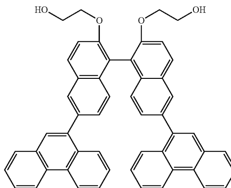
9DPNBINOL-2EO 2,2'-bis(2-hydroxyethoxy)-6,6'- di(phenanthrene-9-yl)-1,1'-binaphthalene
