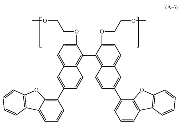
[Chemical Formula 11]
