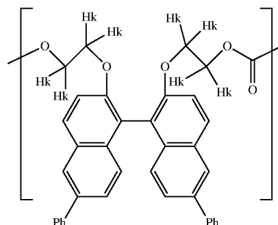
[Chemical Formula 40]
