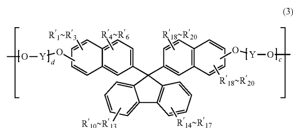
[Chemical Formula 31]
