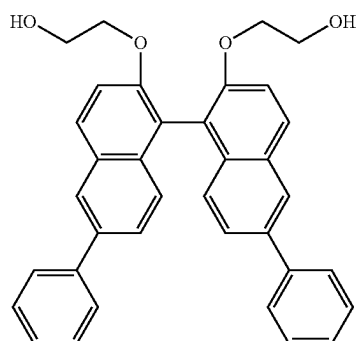
BINL-2EO-2,2'-bis(2-hydroxyethoxy)- 6,6'-diphenyl-1,1'-binaphthalene
