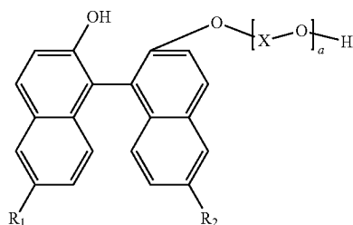
[Chemical Formula 35]
