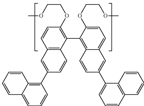
[Chemical Formula 25]
