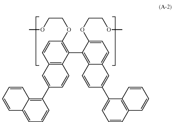
[Chemical Formula 7]
