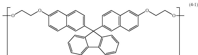
[Chemical Formula 16]
