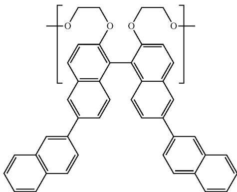
[Chemical Formula 26]
