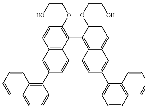
DNBINOL-2EO 2,2'-bis(2-hydroxyethoxy)-6,6'- di(naphthalene-1-yl)-1,1'-binaphthalene
