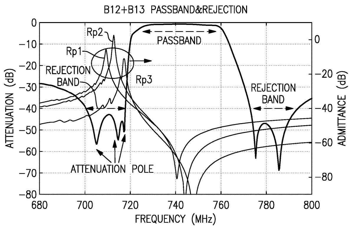
FIG.8 (PRIOR ART)
