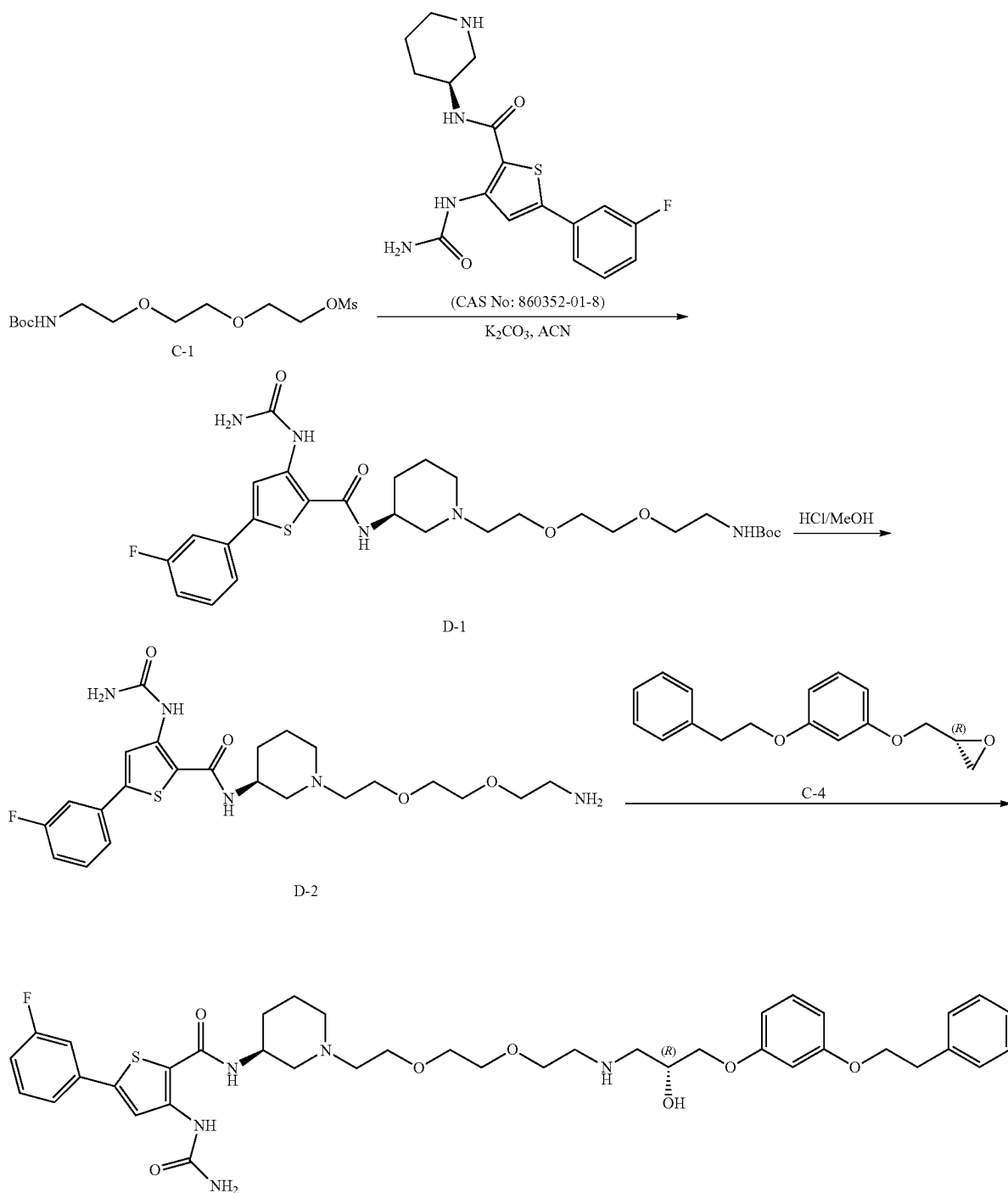
Compound D
