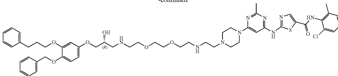
Compound E
