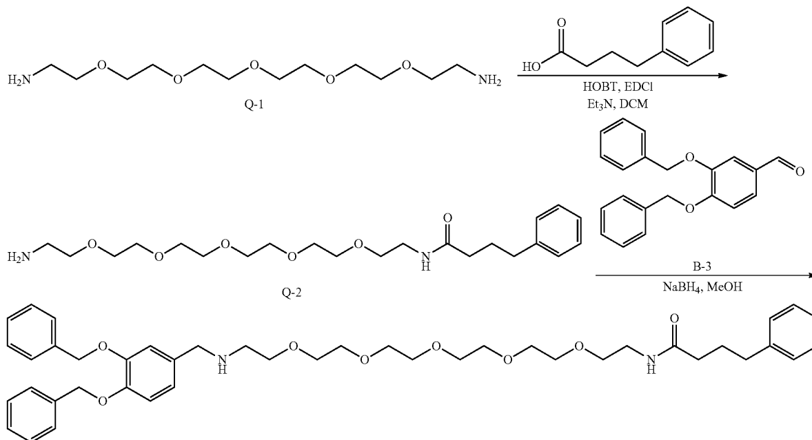
Compound Q
