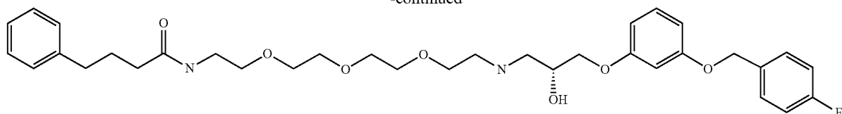
Compound T
