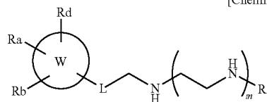
[Chemical Formula 1]
