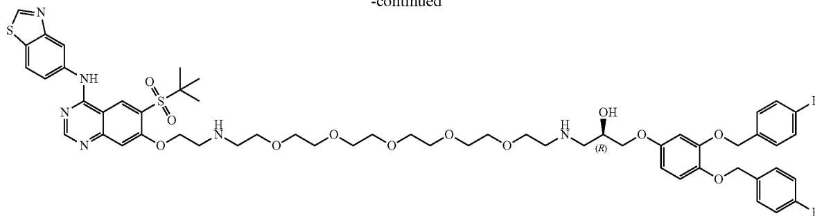
Compound P
