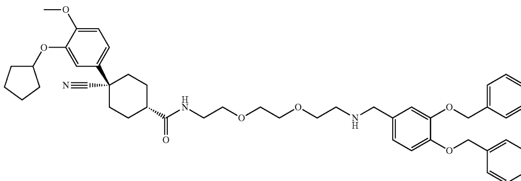
Compound B
