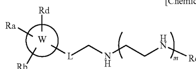
[Chemical Formula 1]
