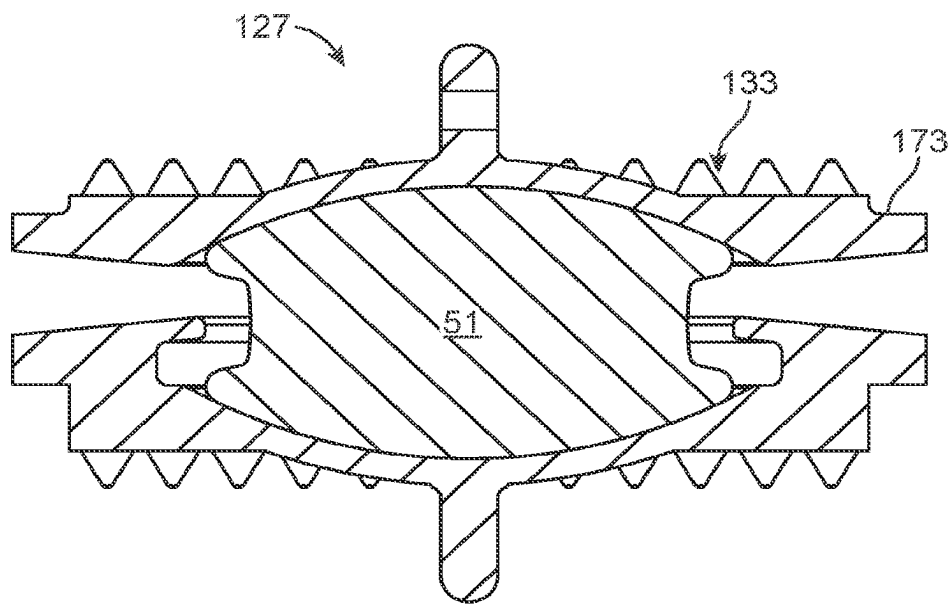
FIG. 5 (PRIOR ART)
