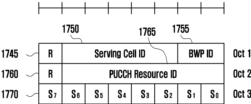
PUCCH spatial relation Activation/Deactivation MAC CE
