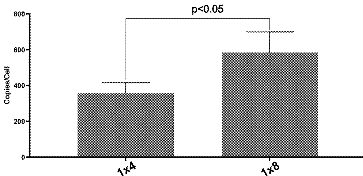
Target Denisty in Matched Expression A*11:01 K562 Engineered Lines
