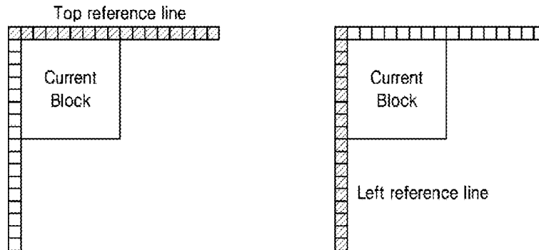
(a) Top reference sample line and left reference sample line
