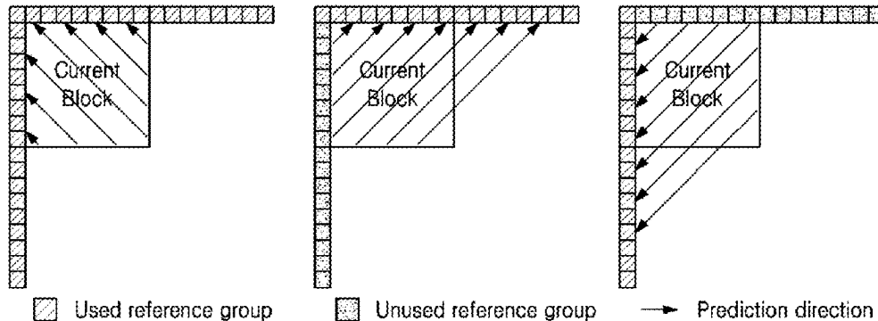
(b) Use of reference sample group according to intra-prediction
