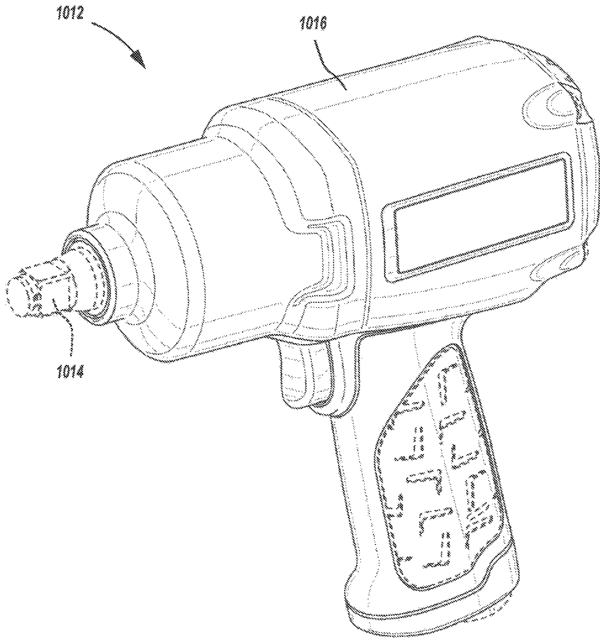
FIG. 2 (Prior Art)
