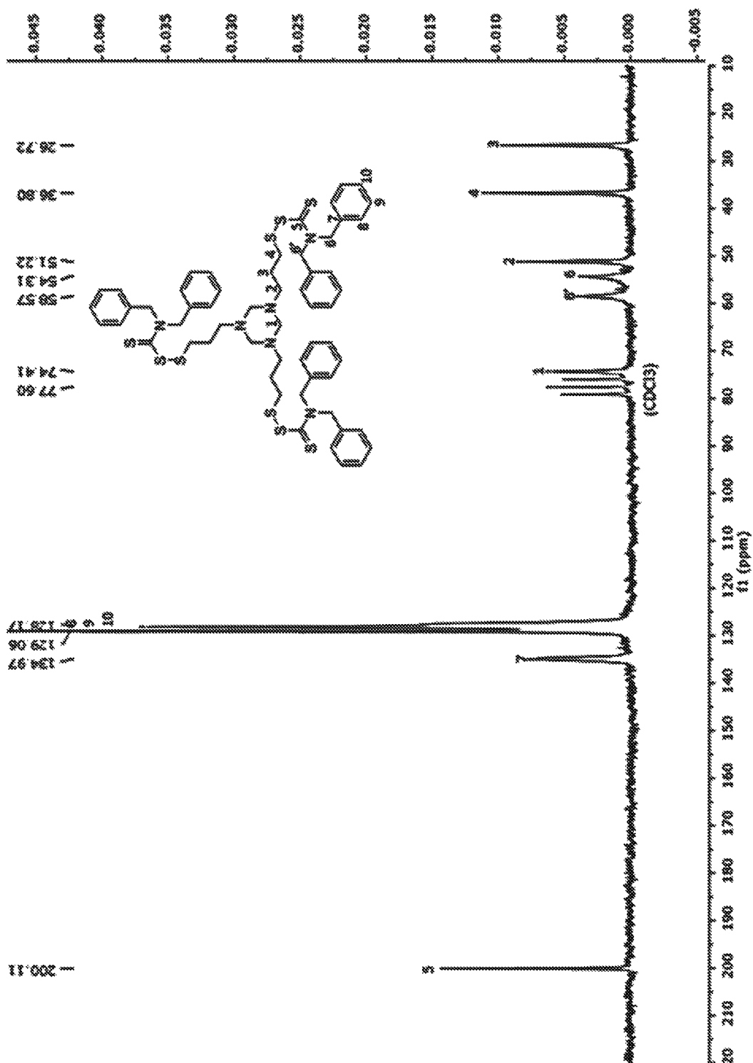
Figure 1 (carbon 13 NMR spectrum):
