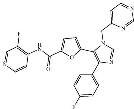
5-(4-(4-fluorophenyl)-1-(pyrimidin-4-ylmethyl)-1H-imidazol-5-yl)-N-(3-fluoropyridin-4-yl)furan-2-carboxamide
