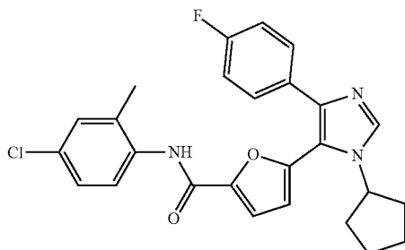
N-(4-chloro-2-methylphenyl)-5-(1-cyclopentyl-4-(4-fluorophenyl)-1H-imidazol-5-yl)furan-2-carboxamide
