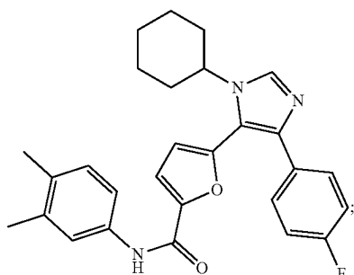
5-(1-cyclohexyl-4-(4-fluorophenyl)-1H-imidazol-5-yl)-N-(3,4-dimethylphenyl)furan-2-carboxamide
