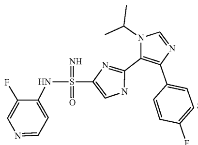
5'-(4-fluorophenyl)-N-(3-fluoropyridin-4-yl)-3'-isopropyl-1H,3'H-[2,4'-biimidazole]-4-sulfonimidamide
