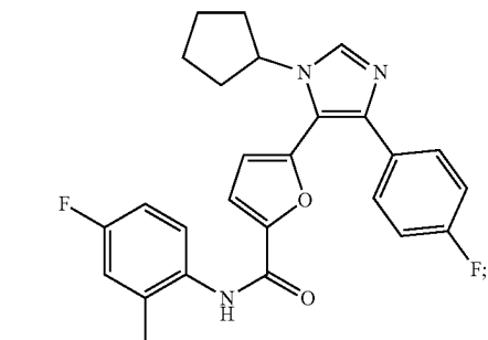
5-(1-cyclopentyl-4-(4-fluorophenyl)-1H-imidazol-5-yl)-N-(4-fluoro-2-methylphenyl)furan-2-carboxamide
