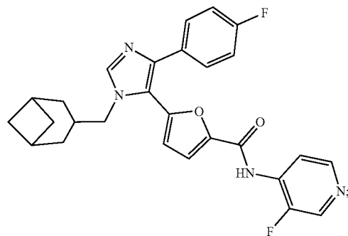
5-(1-bicyclo[3.1.1]heptan-3-ylmethyl)-4-(4-fluorophenyl)-1H-imidazol-5-yl)-N-(3-fluoropyridin-4-yl)furan-2-carboxamide
