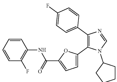
5-(1-cyclopentyl-4-(4-fluorophenyl)-1H-imidazol-5-yl)-N-(2-fluorophenyl)furan-2-carboxamide
