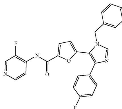
5-(1-(1-benzyl)-4-(4-fluorophenyl)-1H-imidazol-5-yl)-N-(3-fluoropyridin-4-yl)furan-2-carboxamide
