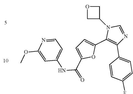
5-(4-(4-fluorophenyl)-1-(oxetan-3-yl)-1H-imidazol-5-yl)-N-(2-methoxy pyridin-4-yl)furan-2-carboxamide
