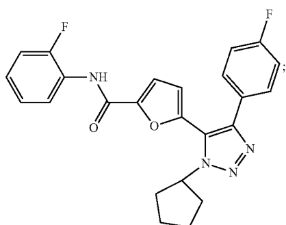
5-(1-cyclopentyl-4-(4-fluorophenyl)-1H-1,2,3-triazol-5-yl)-N-(2-fluorophenyl)furan-2-carboxamide
