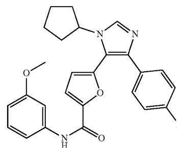
5-(1-cyclopentyl-4-(4-fluorophenyl)-1H-imidazol-5-yl)-N-(3-methoxyphenyl)furan-2-carboxamide
