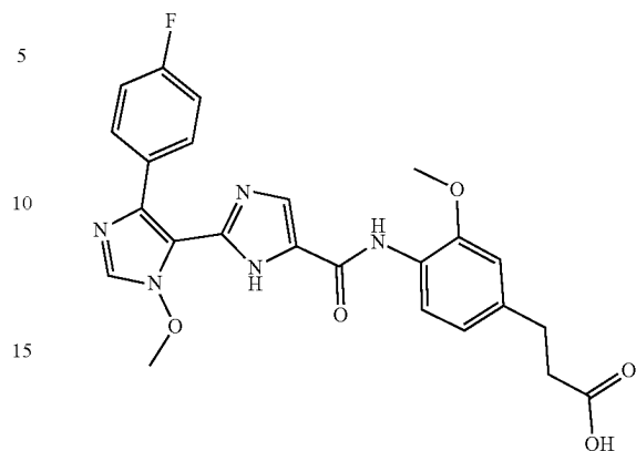
3-(4-(5'-(4-fluorophenyl)-3'-methoxy-1H,3'H-[2,4'-biimidazole]-5-carboxamido)-3-methoxyphenyl)propanoic acid
