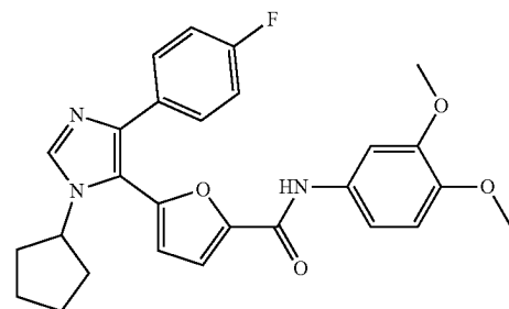
5-(1-cyclopentyl-4-(4-fluorophenyl)-1H-imidazol-5-yl)-N-(3,4-dimethoxyphenyl)furan-2-carboxamide
