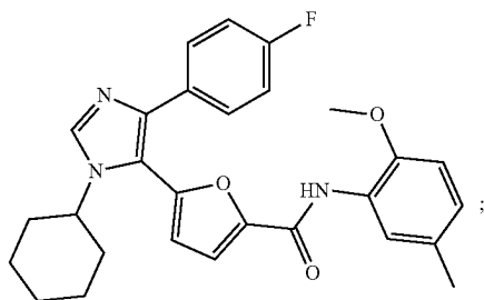
5-(1-cyclohexyl-4-(4-fluorophenyl)-1H-imidazol-5-yl)- N-(2-methoxy-5-methylphenyl)furan-2-carboxamide
