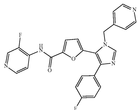
5-(4-(4-fluorophenyl)-1-(pyridin-4-ylmethyl)-1H-imidazol-5-yl)-N-(3-fluoropyridin-4-yl)furan-2-carboxamide
