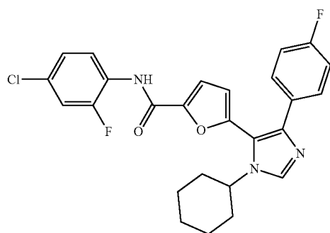
N-(4-chloro-2-fluorophenyl)-5-(1-cyclohexyl-4-(4-fluorophenyl)-1H-imidazol-5-yl)furan-2-carboxamide
