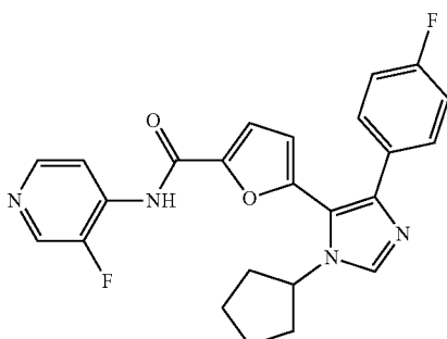
5-(1-cyclopentyl-4-(4-fluorophenyl)-1H-imidazol-5-yl)- N-(3-fluoropyridin-4-yl)furan-2-carboxamide
