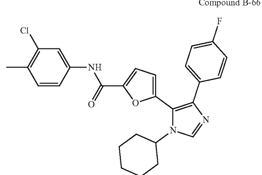
N-(3-chloro-4-methylphenyl)-5-(1-cyclohexyl-4-(4-fluorophenyl)-1H-imidazol-5-yl)furan-2-carboxamide
