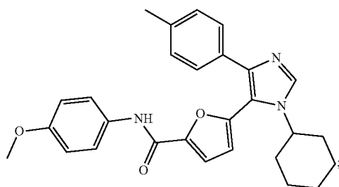
5-(1-cyclohexyl-4-(p-tolyl)-1H-imidazol-5-yl)-N-(4-methoxyphenyl)furan-2-carboxamide
