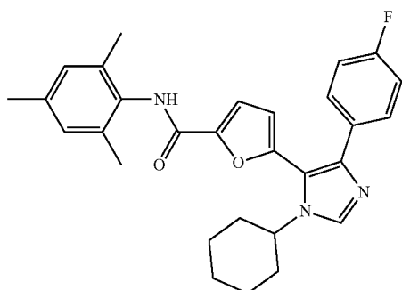
5-(1-cyclohexyl-4-(4-fluorophenyl)-1H-imidazol-5-yl)-N-mesitylfuran-2-carboxamide
