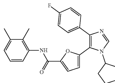
5-(1-cyclopentyl-4-(4-fluorophenyl)-1H-imidazol-5-yl)-N-(2,3-dimethylphenyl)furan-2-carboxamide
