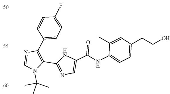
3'-(tert-butyl)-N-(2-chloro-4-(2-hydroxyethyl)phenyl)-5'-(4-fluorophenyl)-1H,3'H-[2,4'-biimidazole]-5-carboxamide
