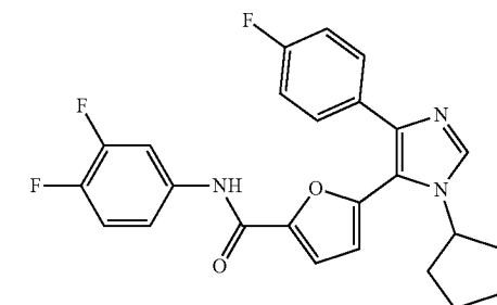
5-(1-cyclopentyl-4-(4-fluorophenyl)-1H-imidazol-5-yl)-N-(3,4-difluorophenyl)furan-2-carboxamide
