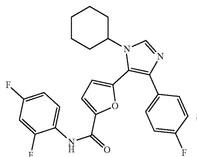
5-(1-cyclohexyl-4-(4-fluorophenyl)-1H-imidazol- 5-yl)-N-(2,4-difluorophenyl)furan-2-carboxamide
