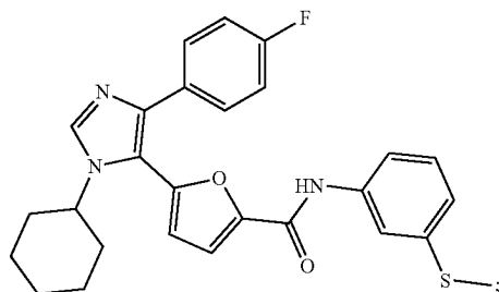
5-(1-cyclohexyl-4-(4-fluorophenyl)-1H-imidazol-5-yl)-N-(3-(methylthio)phenyl)furan-2-carboxamide
