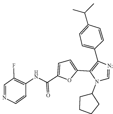
5-(1-cyclopentyl-4-(4-isopropylphenyl)-1H-imidazol-5-yl)-N-(3-fluoropyridin-4-yl)furan-2-carboxamide
