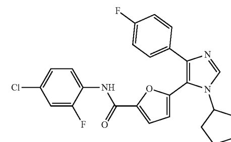
N-(4-chloro-2-fluorophenyl)-5-(1-cyclopentyl-4-(4-fluorophenyl)-1H-imidazol-5-yl)furan-2-carboxamide
