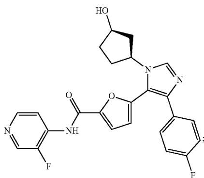
rac-5-(4-(4-fluorophenyl)-1-((1R,3S)-3-hydroxycyclopentyl)-1H-imidazol-5-yl)-N-(3-fluoropyridin-4-yl)furan-2-carboxamide
