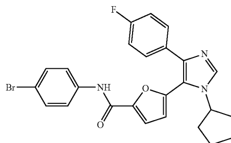
N-(4-bromophenyl)-5-(1-cyclopentyl-4-(4-fluorophenyl)-1H-imidazol-5-yl)furan-2-carboxamide
