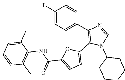
5-(1-cyclohexyl-4-(4-fluorophenyl)-1H-imidazol-5- yl)-N-(2,6-dimethylphenyl)furan-2-carboxamide
