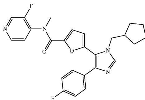
5-(1-(cyclopentylmethyl)-4-(4-fluorophenyl)-1H-imidazol-5-yl)-N-(3-fluoropyridin-4-yl)-N-methylfuran-2-carboxamide
