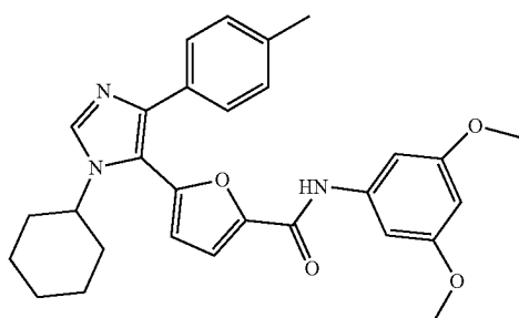
5-(1-cyclohexyl-4-(p-tolyl)-1H-imidazol-5-yl)-N-(3,5-dimethoxyphenyl)furan-2-carboxamide
