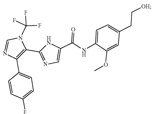
5'-(4-fluorophenyl)-N-(4-(2-hydroxyethyl)-2-methoxyphenyl)-3'-trifluoromethyl-1H,3'H-[2,4'-biimidazole]-5-carboxamide
