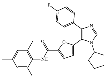
5-(1-cyclopentyl-4-(4-fluorophenyl)-1H-imidazol-5-yl)-N-mesitylfuran-2-carboxamide
