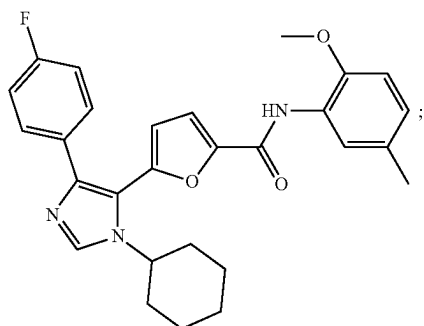
5-(1-cyclohexyl-4-(4-fluorophenyl)-1H-imidazol-5-yl)-N-(2-methoxy-5-methylphenyl)furan-2-carboxamide
