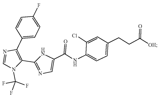
3-(3-chloro-4-(5'-(4-fluorophenyl)-3'-(trifluoromethyl)-1H,3'H-[2,4'-biimidazole]-5-carboxamido)phenyl)propanoic acid
