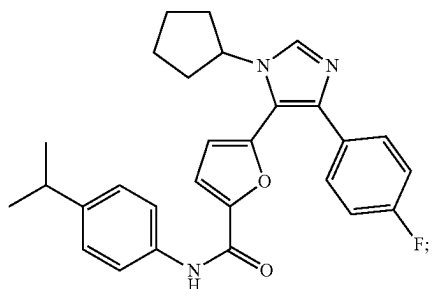
5-(1-cyclopentyl-4-(4-fluorophenyl)-1H-imidazol-5-yl)-N-(4-isopropylphenyl)furan-2-carboxamide
