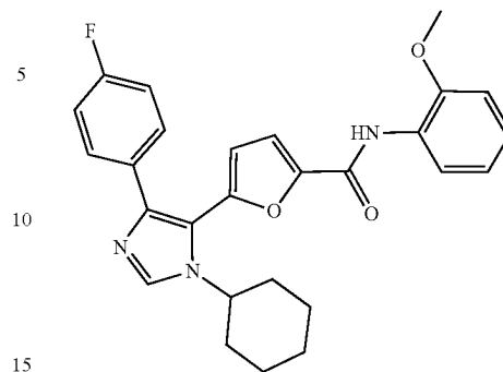
5-(1-cyclohexyl-4-(4-fluorophenyl)-1H-imidazol-5-yl)-N-(2-methoxyphenyl)furan-2-carboxamide
