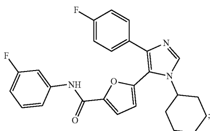
5-(1-cyclohexyl-4-(4-fluorophenyl)-1H-imidazol-5-yl)-N-(3-fluorophenyl)furan-2-carboxamide
