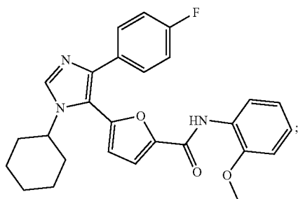
5-(1-cyclohexyl-4-(4-fluorophenyl)-1H-imidazol-5-yl)-N-(2-methoxyphenyl)furan-2-carboxamide
