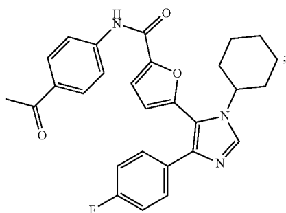
N-(4-acetylphenyl)-5-(1-cyclohexyl-4-(4-fluorophenyl)-1H-imidazol-5-yl)furan-2-carboxamide
