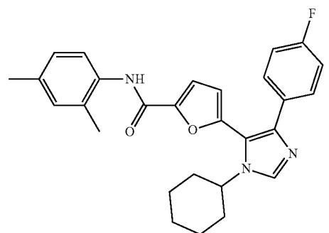
5-(1-cyclohexyl-4-(4-fluorophenyl)-1H-imidazol-5-yl)-N-(2,4-dimethylphenyl)furan-2-carboxamide
