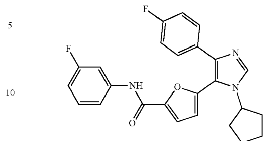
5-(1-cyclopentyl-4-(4-fluorophenyl)-1H-imidazol-5-yl)-N-(3-fluorophenyl)furan-2-carboxamide
