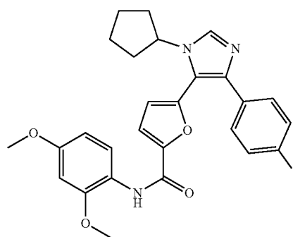
5-(1-cyclopentyl-4-(4-fluorophenyl)-1H-imidazol-5-yl)-N-(2,4-dimethoxyphenyl)furan-2-carboxamide
