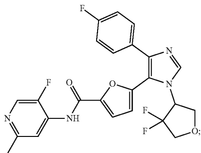
5-(1-(4,4-difluorotetrahydrofuran-3-yl)-4-(4-fluorophenyl)-1H-imidazol-5-yl)-N-(5-fluoro-2-methylpyridin-4-yl)furan-2-carboxamide
