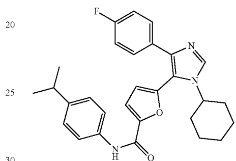
5-(1-cyclohexyl-4-(4-fluorophenyl)-1H-imidazol-5-yl)-N-(4-isopropylphenyl)furan-2-carboxamide
