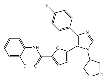
N-(2-fluorophenyl)-5-(4-(4-fluorophenyl)-1-(tetrahydrofuran-3-yl)-1H-imidazol-5-yl)furan-2-carboxamide
