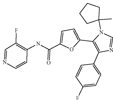
5-(4-(4-fluorophenyl)-1-(1-methylcyclopentyl)-1H-imidazol-5-yl)-N-(3-fluoropyridin-4-yl)furan-2-carboxamide
