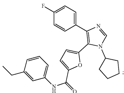
5-(1-cyclopentyl-4-(4-fluorophenyl)-1H-imidazol-5-yl)-N-(3-ethylphenyl)furan-2-carboxamide
