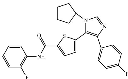
5-(1-cyclopentyl-4-(4-fluorophenyl)-1H-imidazol-5-yl)- N-(2-fluorophenyl)thiophene-2-carboxamide
