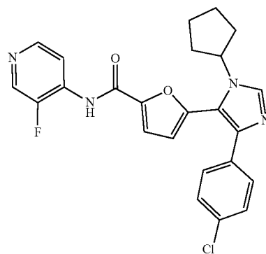
5-(4-(4-chlorophenyl)-1-cyclopentyl-1H-imidazol-5-yl)-N-(3-fluoropyridin-4-yl)furan-2-carboxamide
