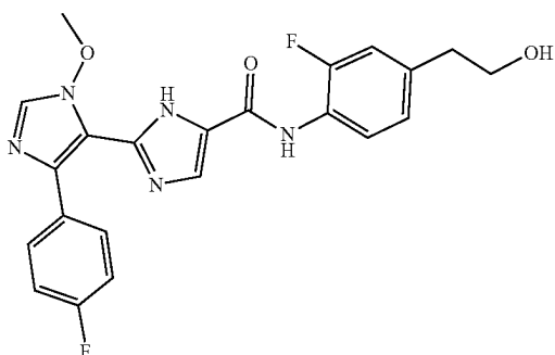
N-(2-fluoro-4-(2-hydroxyethyl)phenyl)-5'-(4-fluorophenyl)-3'-methoxy-1H,3'H-[2,4'-biimidazole]-5-carboxamide
