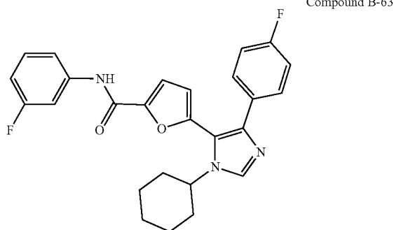
5-(1-cyclohexyl-4-(4-fluorophenyl)-1H-imidazol-5-yl)-N-(3-fluorophenyl)furan-2-carboxamide
