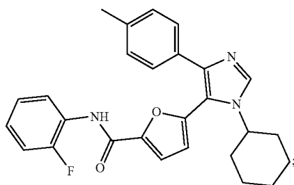
5-(1-cyclohexyl-4-(p-tolyl)-1H-imidazol-5-yl)-N-(2-fluorophenyl)furan-2-carboxamide
