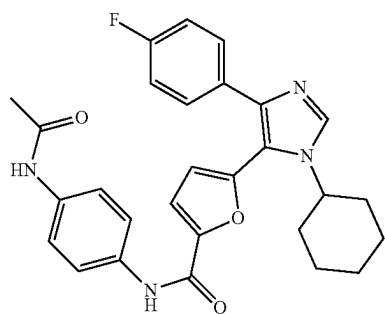
N-(4-acetamidophenyl)-5-(1-cyclohexyl-4-(4-fluorophenyl)-1H-imidazol-5-yl)furan-2-carboxamide
