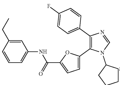
5-(1-cyclopentyl-4-(4-fluorophenyl)-1H-imidazol-5-yl)-N-(3-ethylphenyl)furan-2-carboxamide
