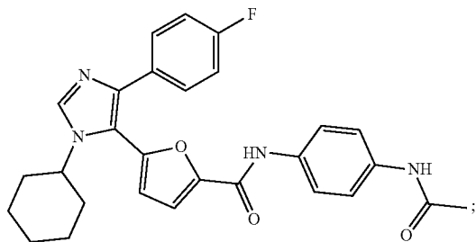
N-(4-acetamidophenyl)-5-(1-cyclohexyl-4-(4-fluorophenyl)-1H- imidazol-5-yl)furan-2-carboxamide
