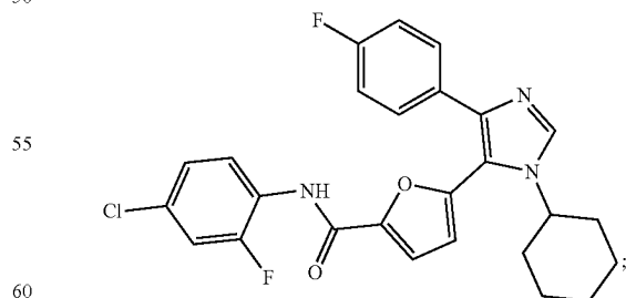
N-(4-chloro-2-fluorophenyl)-5-(1-cyclohexyl-4-(4-fluorophenyl)-1H-imidazol-5-yl)furan-2-carboxamide
