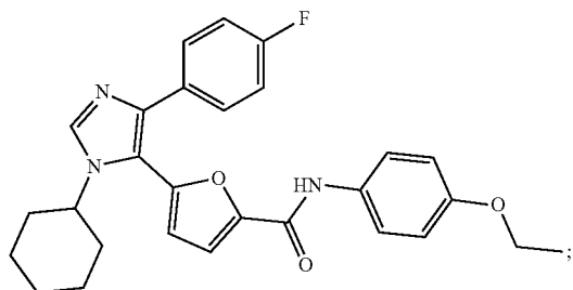
5-(1-cyclohexyl-4-(4-fluorophenyl)-1H-imidazol-5-yl)-N-(4-ethoxyphenyl)furan-2-carboxamide
