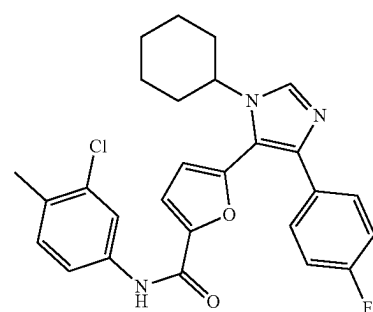
N-(3-chloro-4-methylphenyl)-5-(1-cyclohexyl-4-(4-fluorophenyl)-1H-imidazol-5-yl)furan-2-carboxamide
