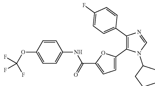
5-(1-cyclopentyl-4-(4-fluorophenyl)-1H-imidazol-5-yl)-N-(4-(trifluoromethoxy)phenyl)furan-2-carboxamide
