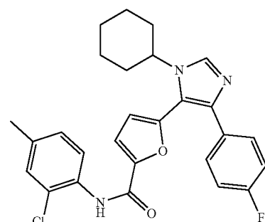
N-(2-chloro-4-methylphenyl)-5-(1-cyclohexyl-4-(4-fluorophenyl)-1H-imidazol-5-yl)furan-2-carboxamide
