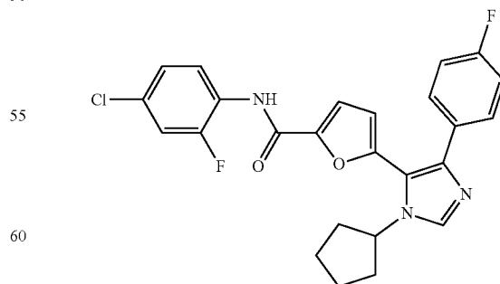
N-(4-chloro-2-fluorophenyl)-5-(1-cyclopentyl-4-(4-fluorophenyl)-1H-imidazol-5-yl)furan-2-carboxamide
