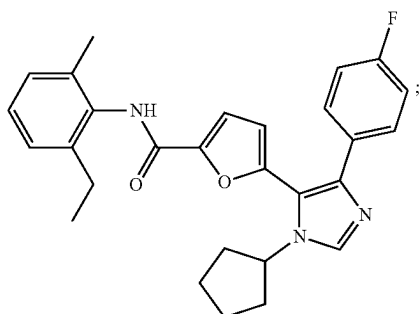
5-(1-cyclopentyl-4-(4-fluorophenyl)-1H-imidazol-5-yl)-N-(2-ethyl-6-methylphenyl)furan-2-carboxamide
