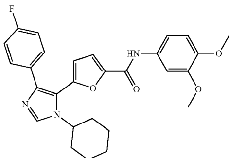
5-(1-cyclohexyl-4-(4-fluorophenyl)-1H-imidazol-5-yl)-N-(3,4-dimethoxyphenyl)furan-2-carboxamide
