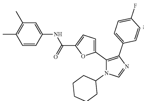
5-(1-cyclohexyl-4-(4-fluorophenyl)-1H-imidazol-5-yl)-N-(3,4-dimethylphenyl)furan-2-carboxamide
