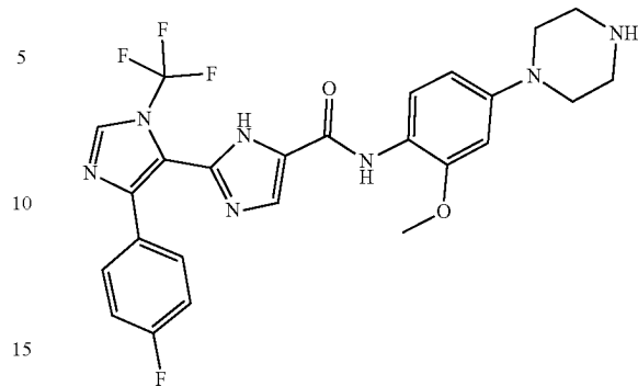
5'-(4-fluorophenyl)-N-(2-methoxy-4-(piperazin-1-yl)phenyl)-3'-trifluoromethyl-1H,3'H-[2,4'-biimidazole]-5-carboxamide
