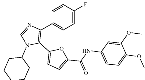
5-(1-cyclohexyl-4-(4-fluorophenyl)-1H-imidazol-5-yl)-N-(3,4-dimethoxyphenyl)furan-2-carboxamide
