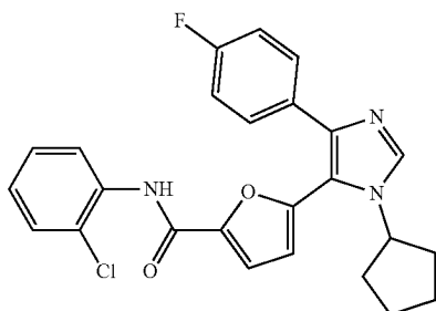
N-(2-chlorophenyl)-5-(1-cyclopentyl-4-(4-fluorophenyl)-1H-imidazol-5-yl)furan-2-carboxamide
