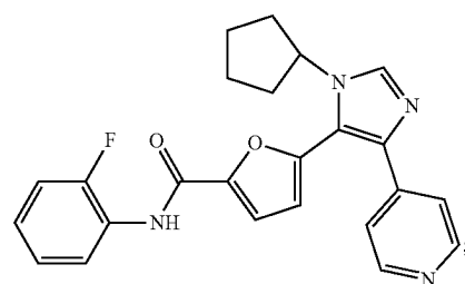
5-(1-cyclopentyl-4-(pyridin-4-yl)-1H-imidazol-5-yl)-N-(2-fluorophenyl)furan-2-carboxamide
