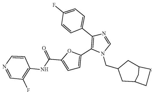
5-(1-bicyclo[3.2.1]octan-3-ylmethyl)-4-(4-fluorophenyl)-1H-imidazol-5-yl)-N-(3-fluoropyridin-4-yl)furan-2-carboxamide
