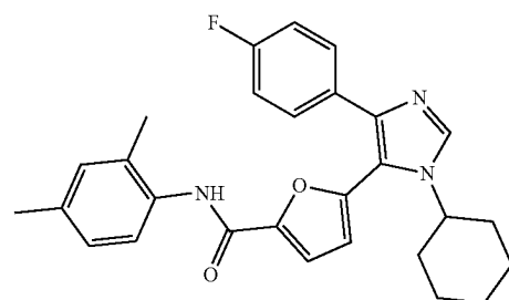
5-(1-cyclohexyl-4-(4-fluorophenyl)-1H-imidazol-5-yl)-N-(2,4-dimethylphenyl)furan-2-carboxamide
