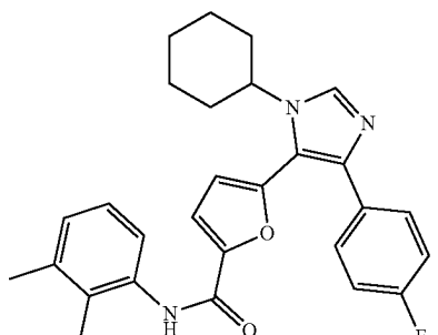
5-(1-cyclohexyl-4-(4-fluorophenyl)-1H-imidazol- 5-yl)-N-(2,3-dimethylphenyl)furan-2-carboxamide
