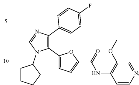
5-(1-cyclopentyl-4-(4-fluorophenyl)-1H-imidazol-5-yl)-N-(3-methoxypyridin-4-yl)furan-2-carboxamide
