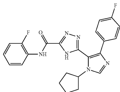
5-(1-cyclopentyl-4-(4-fluorophenyl)-1H-imidazol-5-yl)- N-(2-fluorophenyl)-4H-1,2,4-triazole-3-carboxamide
