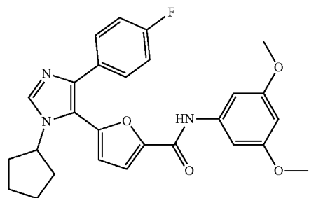
5-(1-cyclopentyl-4-(4-fluorophenyl)-1H-imidazol-5-yl)-N-(3,5-dimethoxyphenyl)furan-2-carboxamide
