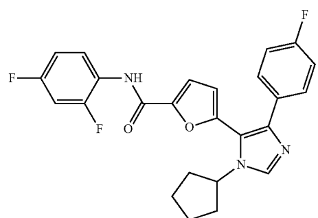
5-(1-cyclopentyl-4-(4-fluorophenyl)-1H-imidazol-5-yl)-N-(2,4-difluorophenyl)furan-2-carboxamide
