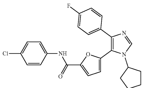
N-(4-chlorophenyl)-5-(1-cyclopentyl-4-(4-fluorophenyl)-1H-imidazol-5-yl)furan-2-carboxamide
