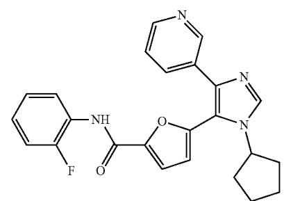
5-(1-cyclopentyl-4-(pyridin-3-yl)-1H-imidazol-5-yl)-N-(2-fluorophenyl)furan-2-carboxamide
