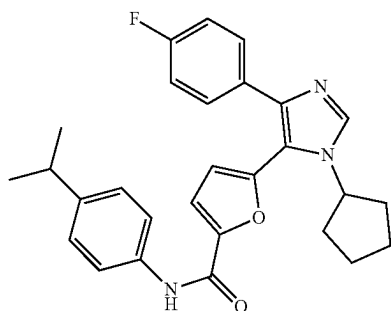
5-(1-cyclopentyl-4-(4-fluorophenyl)-1H-imidazol-5-yl)-N-(4-isopropylphenyl)furan-2-carboxamide
