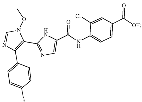
3-chloro-4-(5'-(4-fluorophenyl)-3'-methoxy-1H,3'H-[2,4'-biimidazole]-5-carboxamido)benzoic acid
