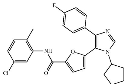
N-(5-chloro-2-methylphenyl)-5-(1-cyclopentyl-4-(4-fluorophenyl)-1H-imidazol-5-yl)furan-2-carboxamide
