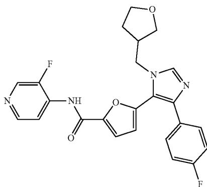
5-(4-(4-fluorophenyl)-1-((tetrahydrofuran-3-yl)methyl)-1H-imidazol-5-yl)-N-(3-fluoropyridin-4-yl)furan-2-carboxamide
