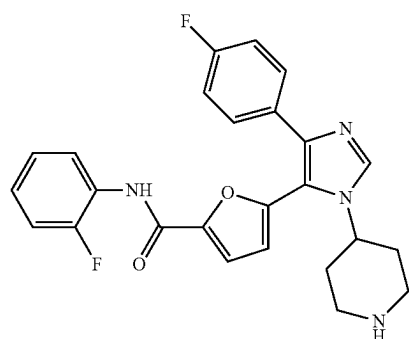
N-(2-fluorophenyl)-5-(4-(4-fluorophenyl)-1-(piperidin-4-yl)-1H-imidazol-5-yl)furan-2-carboxamide
