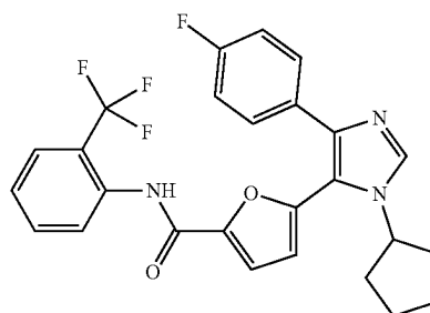
5-(1-cyclopentyl-4-(4-fluorophenyl)-1H-imidazol-5-yl)-N-(2-(trifluoromethyl)phenyl)furan-2-carboxamide
