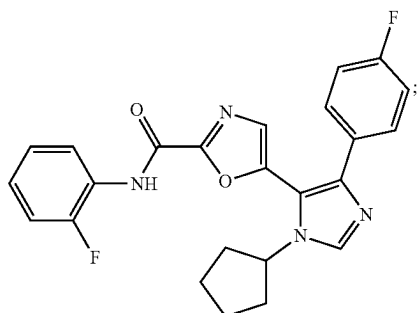
5-(1-cyclopentyl-4-(4-fluorophenyl)-1H-imidazol-5-yl)- N-(2-fluorophenyl)-oxazole-2-carboxamide
