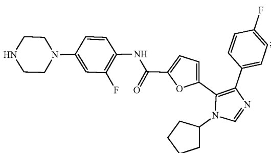
5-(1-(1-cyclopentyl)-4-(4-fluorophenyl)-1H-imidazol-5-yl)-N-(2-fluoro-4-(piperazin-1-yl)phenyl)furan-2-carboxamide
