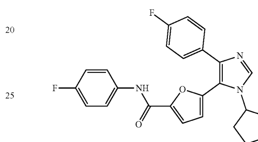
5-(1-cyclopentyl-4-(4-fluorophenyl)-1H-imidazol-5-yl)-N-(4-fluorophenyl)furan-2-carboxamide
