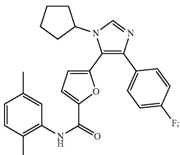
5-(1-cyclopentyl-4-(4-fluorophenyl)-1H-imidazol-5-yl)-N-(2,5-dimethylphenyl)furan-2-carboxamide
