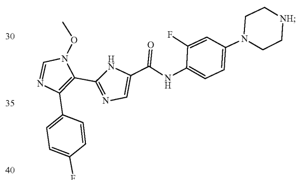
N-(2-fluoro-4-(piperazin-1-yl)phenyl)-5'-(4-fluorophenyl)-3'-methoxy-1H,3'H-[2,4'-biimidazole]-5-carboxamide
