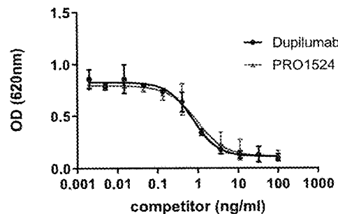
inhibition of IL-4 induced SEAP secretion
