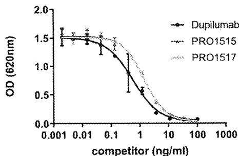
A inhibition of IL-4 induced SEAP secretion
