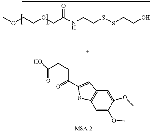
Scheme 7. Synthesis of mPEG 44 -CH 2 CONH-CH 2 CH 2 -SS-CH 2 CH 2 O(O=C)-MSA-2.
