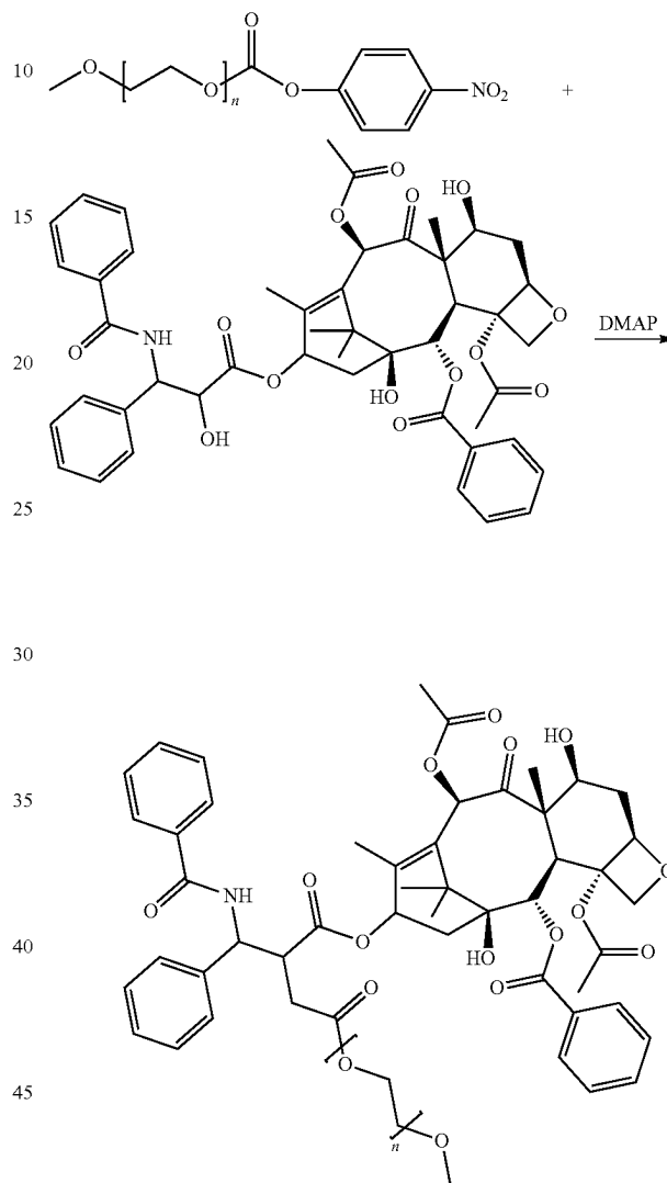
Scheme 2: Synthesis of mPEGn- \text{OCO} -PTX carbonate
