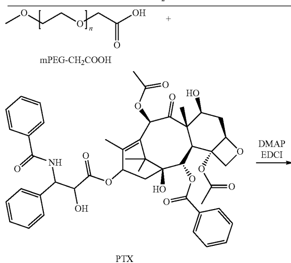
Scheme 1: Esterification reaction of mPEGn-acetic acid with paclitaxel to obtain mPEGn- \text{CH}_2\text{COO} -PTX.
