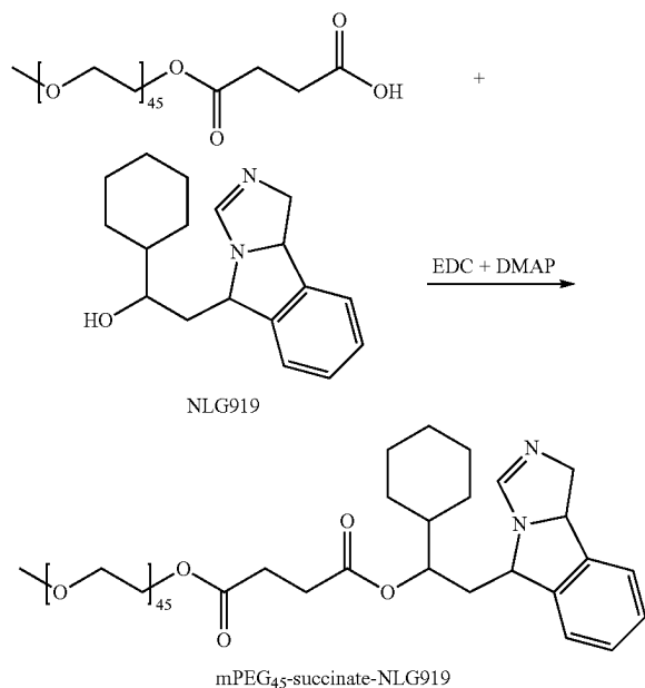
Scheme 9. Synthesis of mPEG 44 -succinate-NLG-919 (IDO-IN-7).
