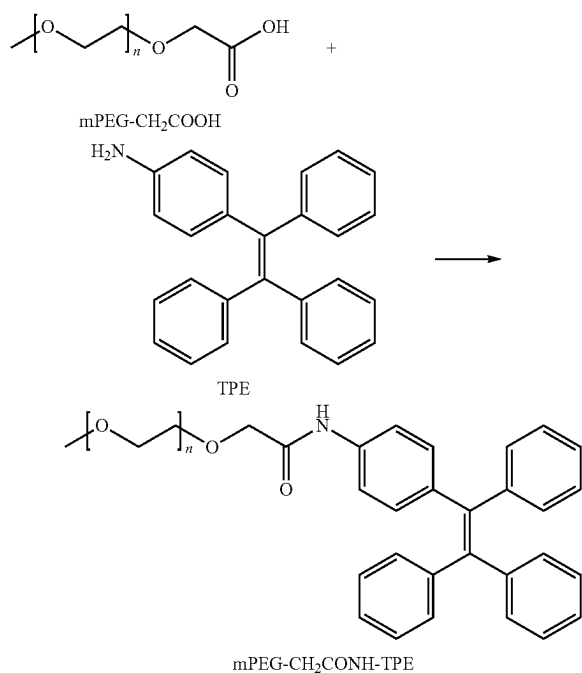
Scheme 5. Synthesis of mPEG-CH 2 -CONH-TPE
