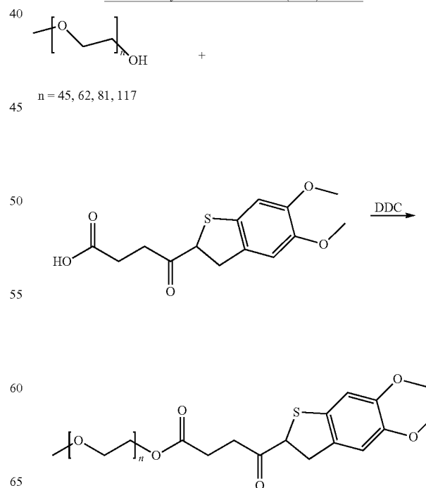
Scheme 6. Synthesis of mPEG n -O(O=C)-MSA-2
