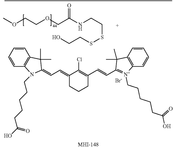
Scheme 10. Synthesis of mPEG 44 -CONH—CH 2 CH 2 SS—CH 2 CH 2 O(O=C)—MHI-148 ester.
