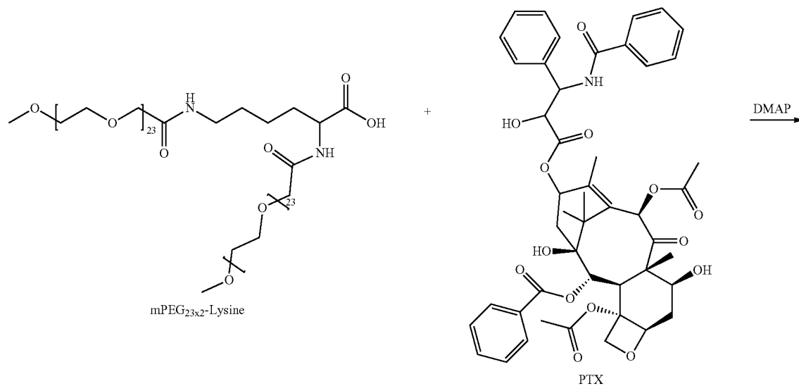
Scheme 4. Synthesis of Monodisperse mPEG 23x2 -Lysine-PTX
