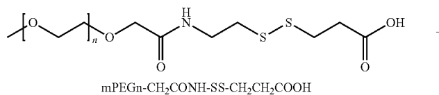
Scheme 3: Synthesis of mPEGn- \text{CH}_2\text{COHN} -SS-CH 2 CH 2 COO-SN38
