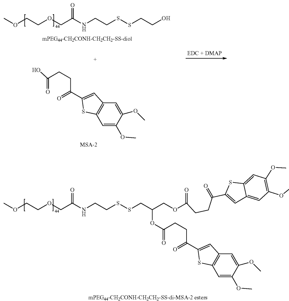
Scheme 8. Synthesis of mPEG 44 -CH 2 CONH-CH 2 CH 2 -SS-di-MSA-2 esters
