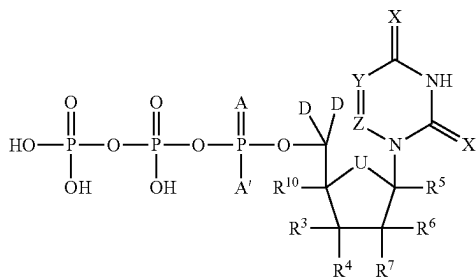
Formula Ie'
