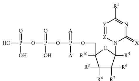
Formula Id
