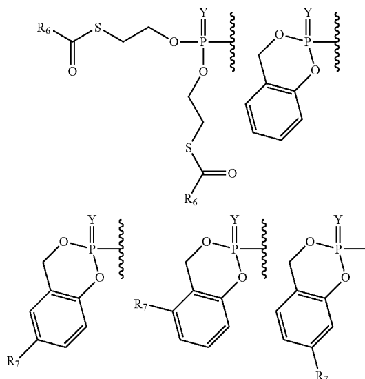
Formula XVIb
