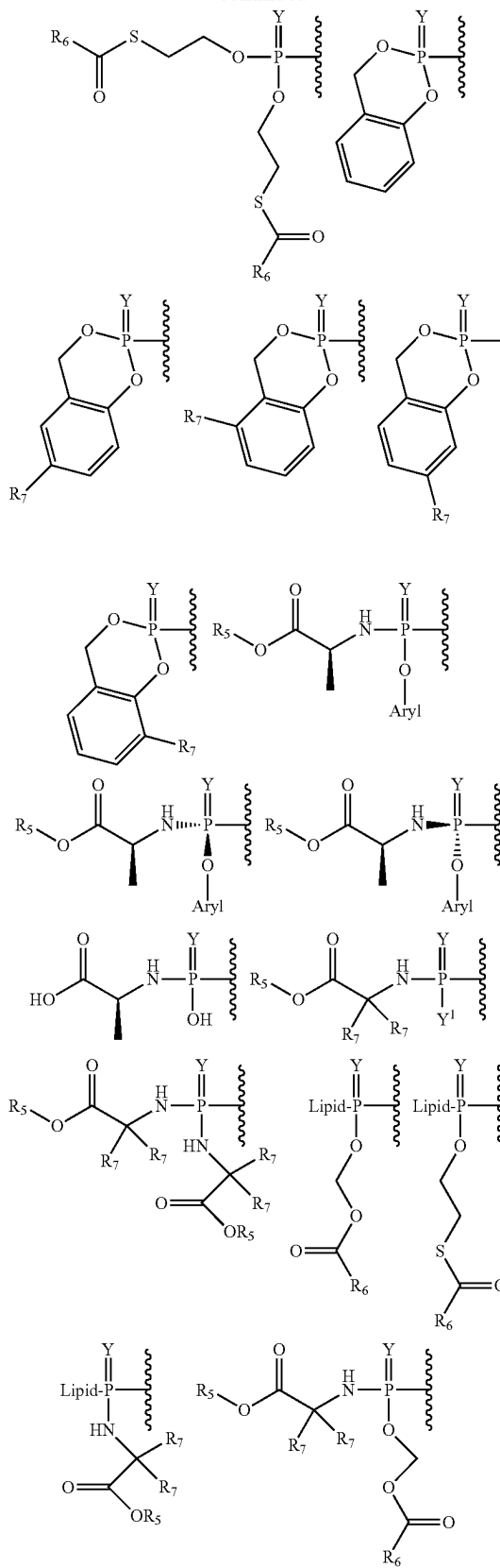
Formula XIVa
