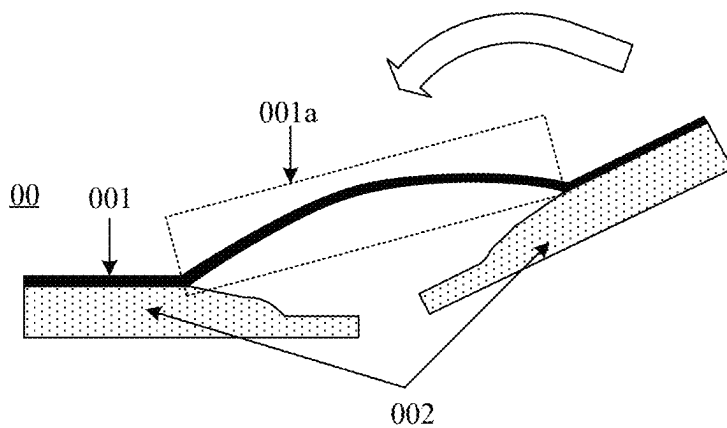
FIG. 2 (Related Art)
