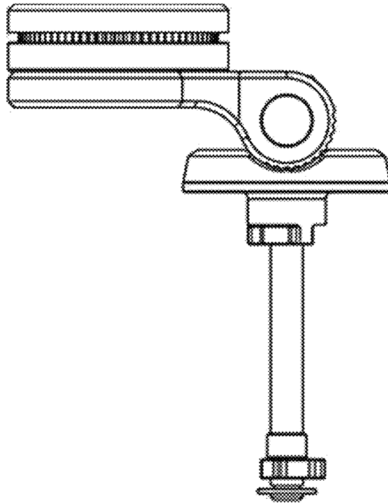
FIG. 2D (prior art)
