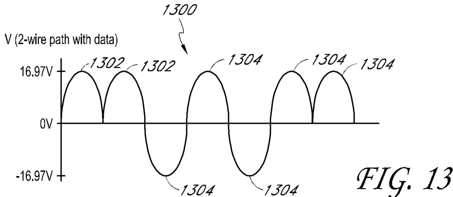
Bridge Waveforms
