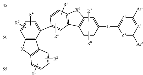
[Chemical Formula 1Cc]
