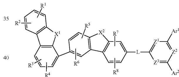
[Chemical Formula 1Cb]
