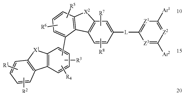
[Chemical Formula 1A]
