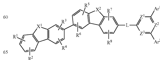
[Chemical Formula 1Cc]
