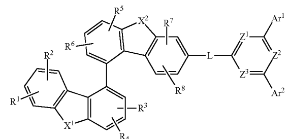
[Chemical Formula 1Ac]
