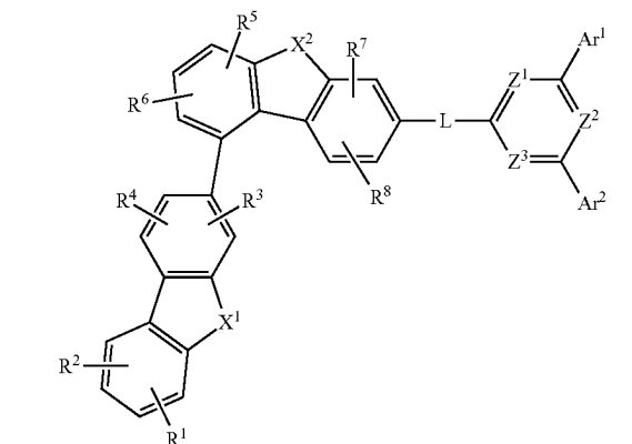
[Chemical Formula 1Ad]
