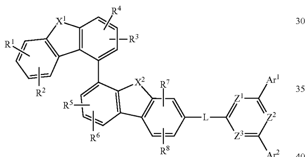
[Chemical Formula 1Bb]
