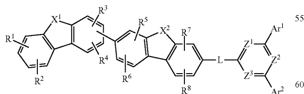
[Chemical Formula 1D]
