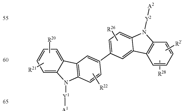
[Chemical Formula 2A-1]
