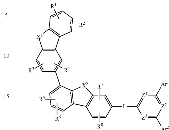
[Chemical Formula 1Bd]
