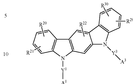
[Chemical Formula 2B-1]
