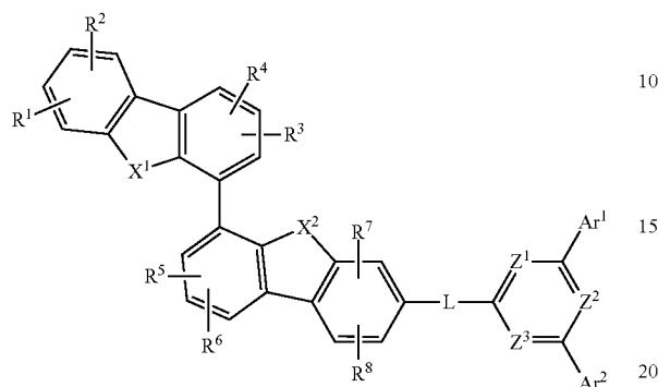
[Chemical Formula 1Ba]
