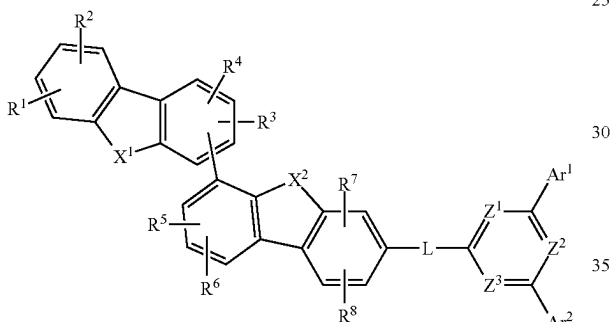
[Chemical Formula 1B]
