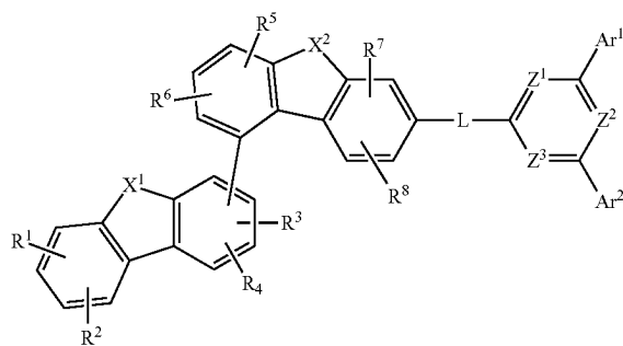
[Chemical Formula 1Ab]
