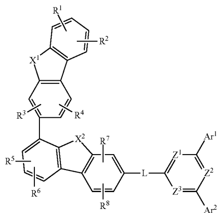
[Chemical Formula 1Bc]
