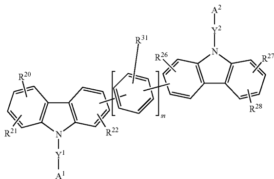
[Chemical Formula 2A]
