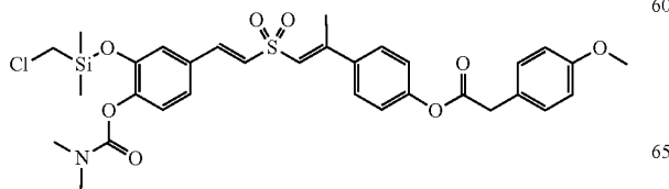
Compound P1-7
