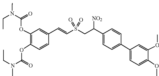
Compound M1-1
