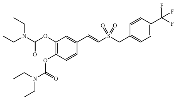
Compound B1-1
