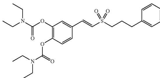
Compound C1-1
