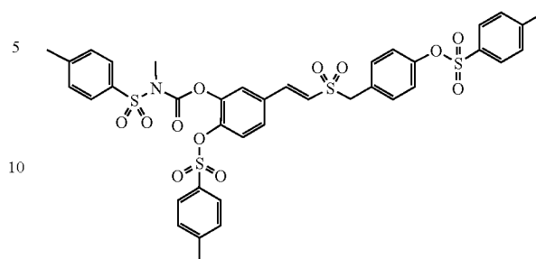
Compound P1-1
