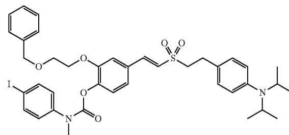
Compound A1-3
