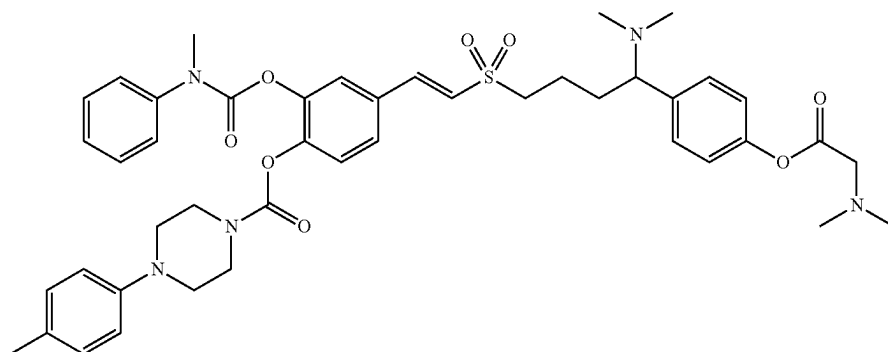
Compound P1-1
