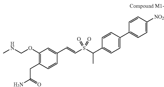
Compound M1-3
