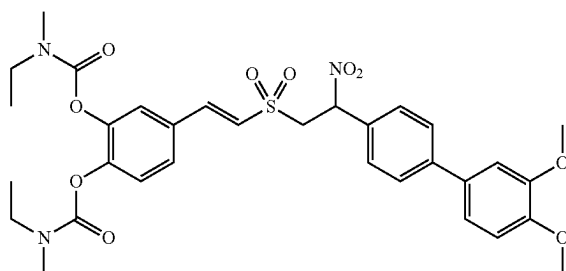
Compound M1-1
