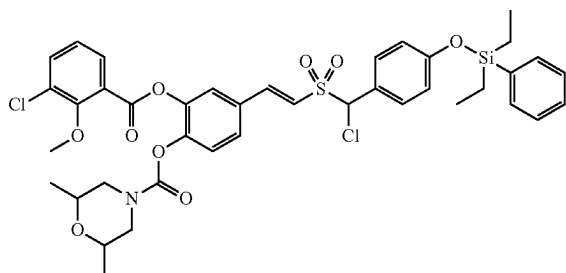
Compound R1-5
