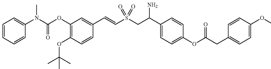
Compound P1-3
