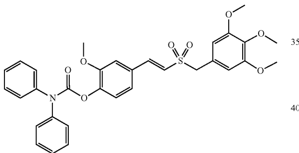
Compound K3-3
