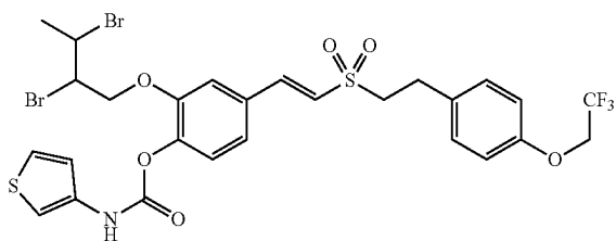
Compound K1-3
