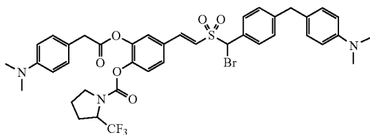
Compound R1-5
