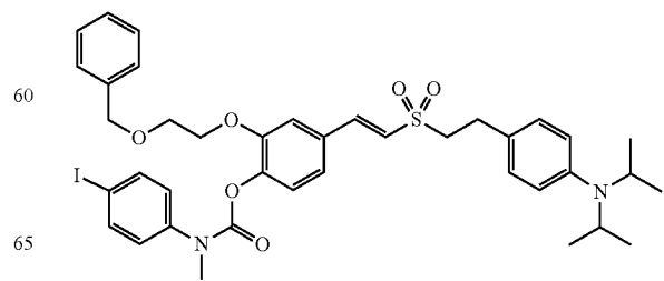
Compound A1-3
