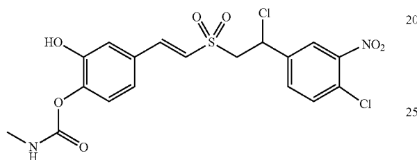
Compound E2-2
