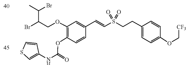
Compound J1-4
