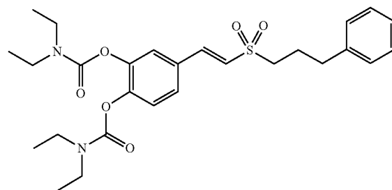
Compound C1-1
