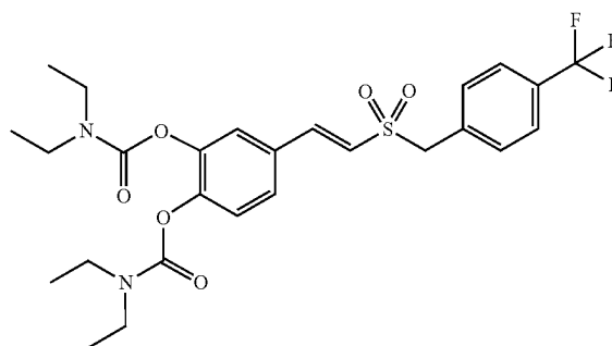
Compound B1-1
