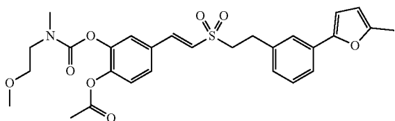
Compound J1-4
