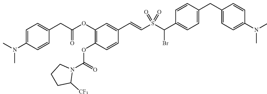
Compound M1-5
