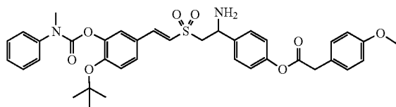
Compound P1-3
