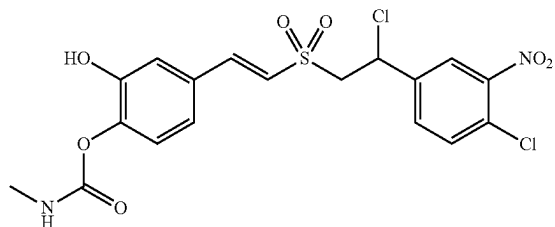
Compound E2-2
