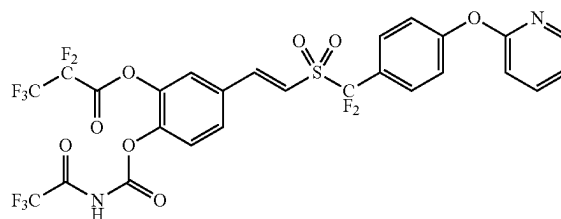
Compound L1-4
