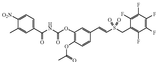
Compound S1-6
