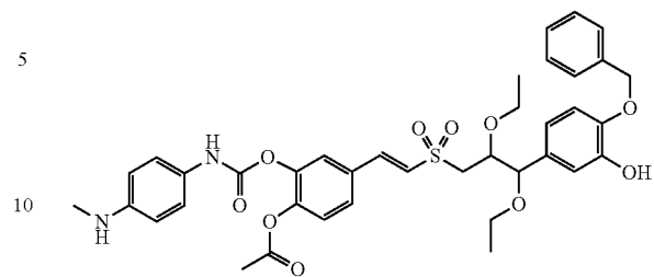
Compound H2-4
