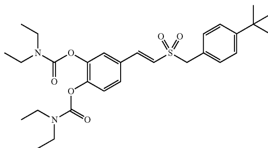
Compound G1-1
