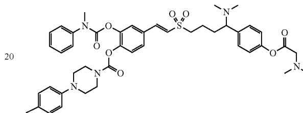
Compound P1-1
