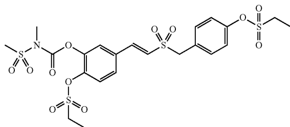
Compound S1-6
