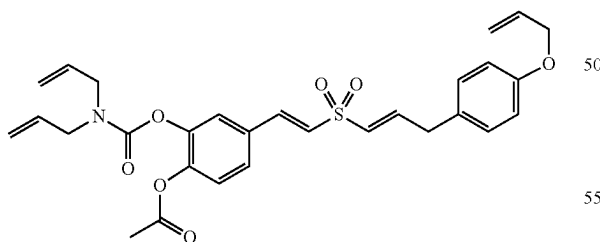
Compound K1-4
