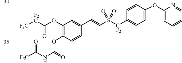
Compound K1-3
