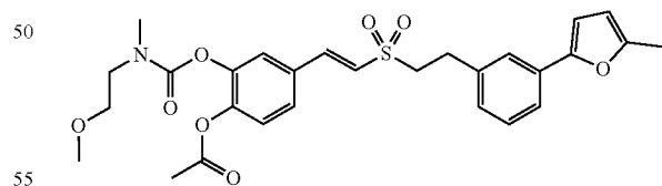
Compound A1-3
