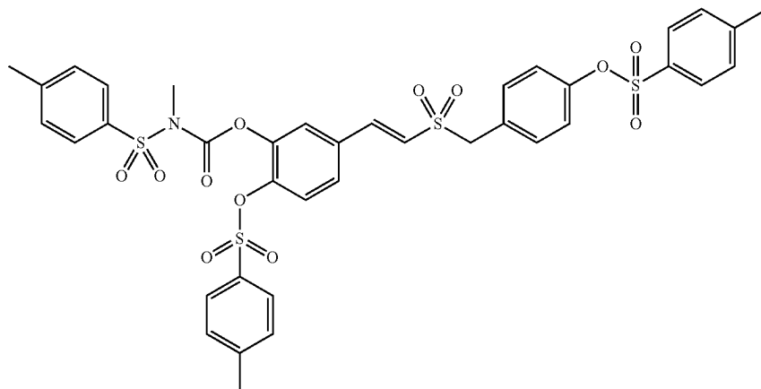
Compound S6-6
