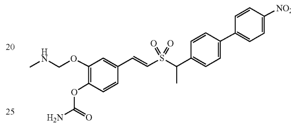
Compound M1-3
