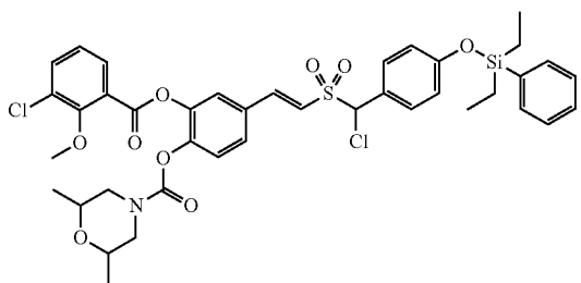
Compound D5-4
