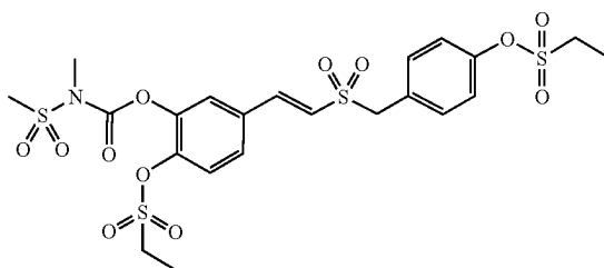
Compound S1-6
