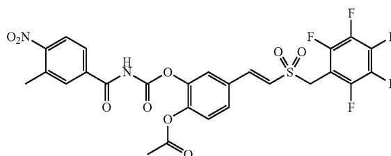
Compound D5-4
