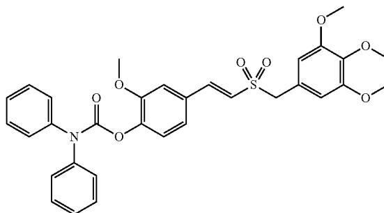
Compound K3-3
