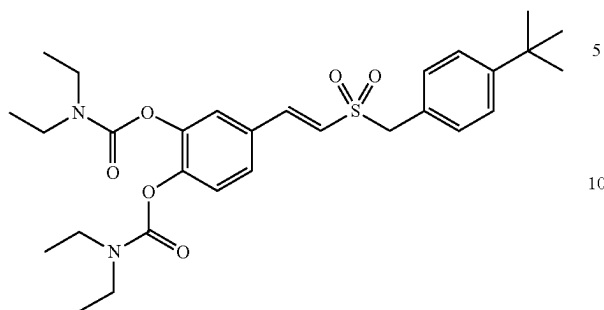
Compound G1-1
