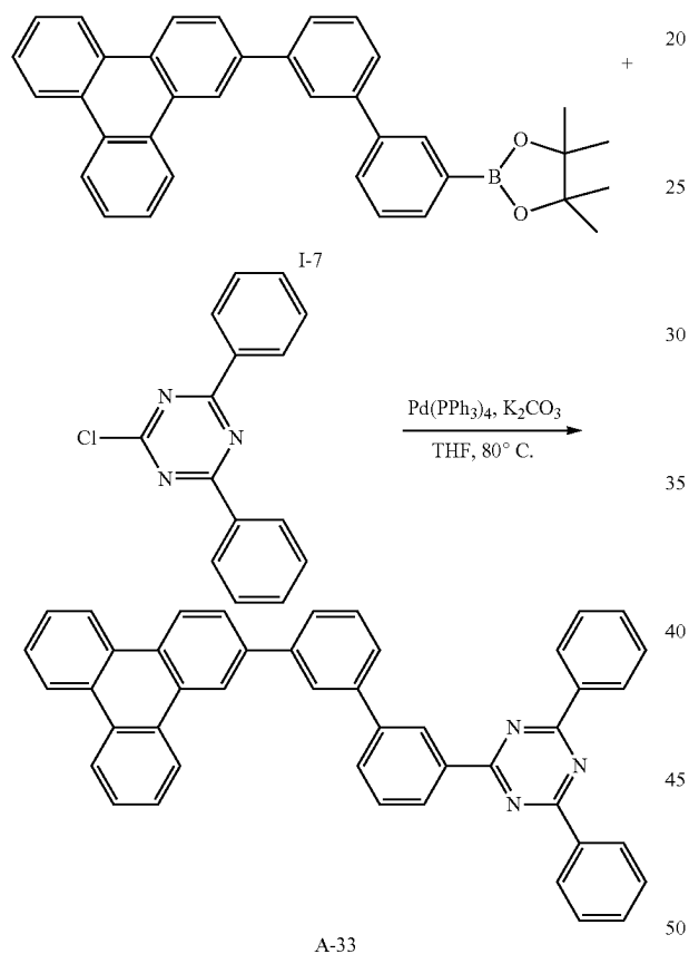
[Reaction Scheme 5]
