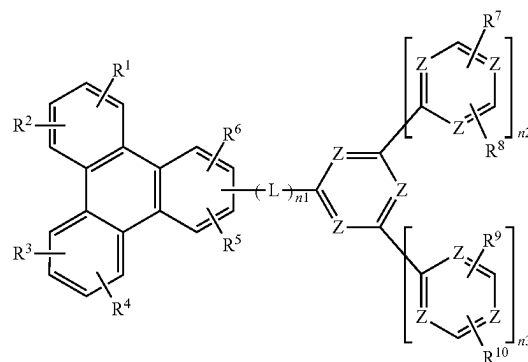
[Chemical Formula 1]
