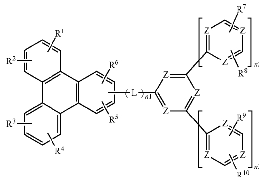
[Chemical Formula 1]
