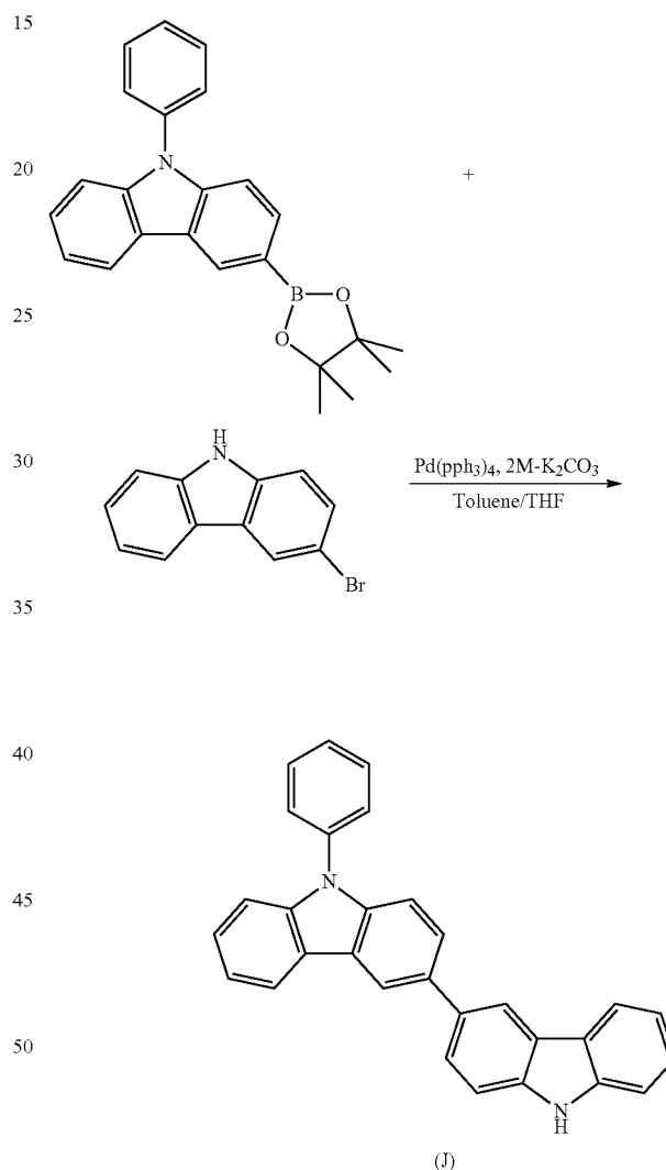
[Reaction Scheme 6]
