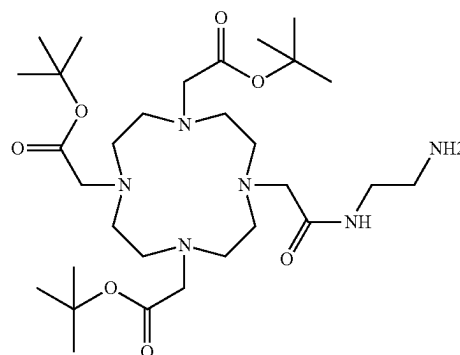
Compound B
