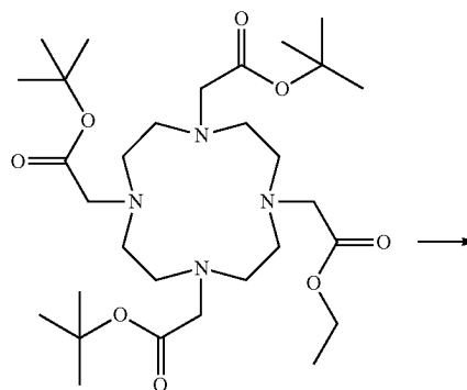
Compound A
