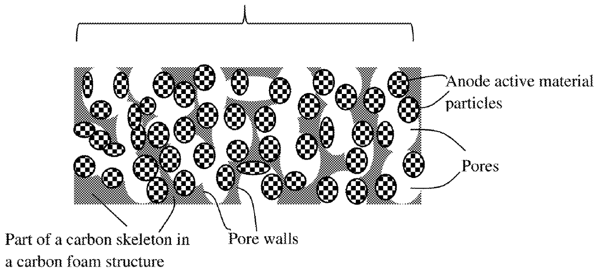
Porous carbon/anode active material composite structure
