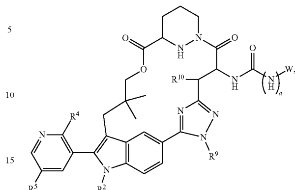
Formula IVb-3
