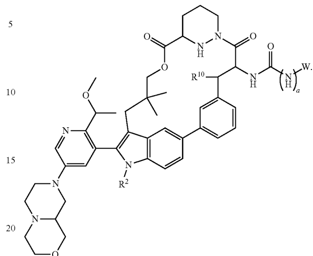
Formula IIIb-9
