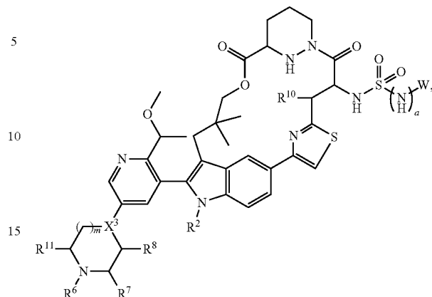
Formula Vb-5
