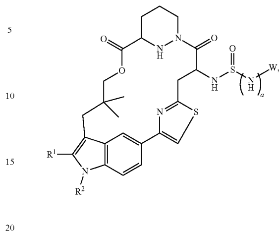
Formula VIIIa
