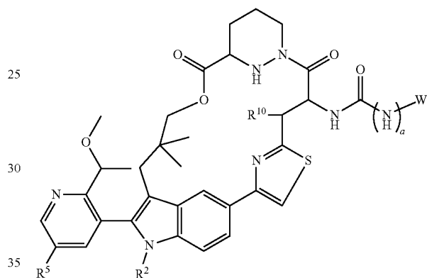
Formula IIb-4
