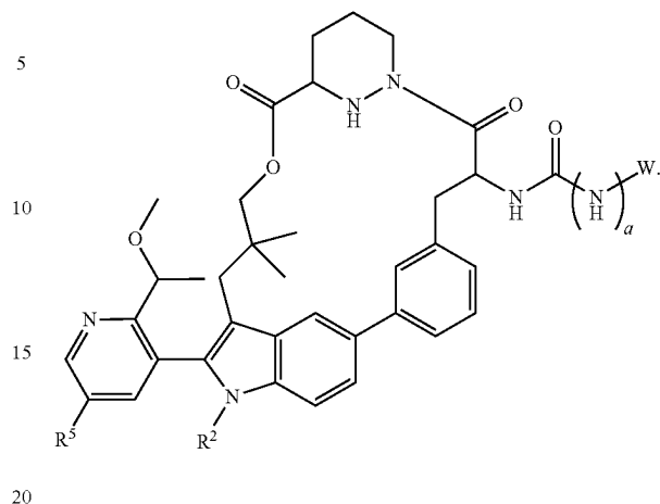
Formula IIIa-4
