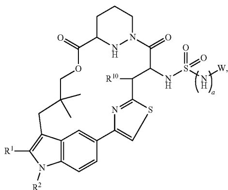
Formula Vb
