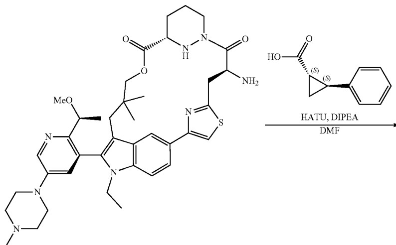
Intermediate 5
