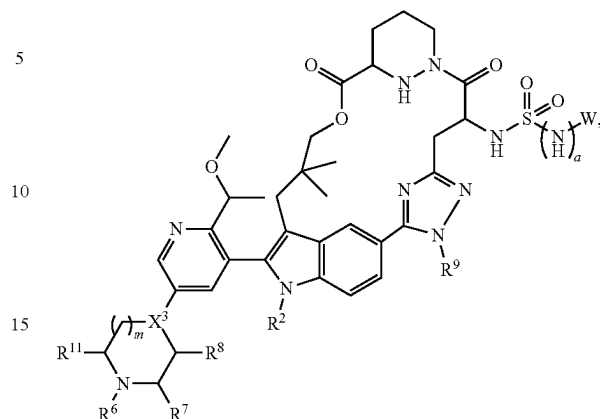
Formula VIIa-5
