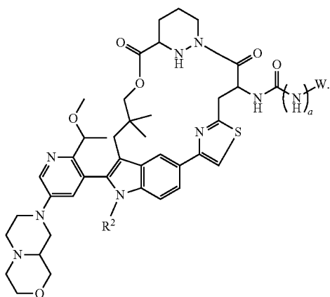
Formula IIa-9
