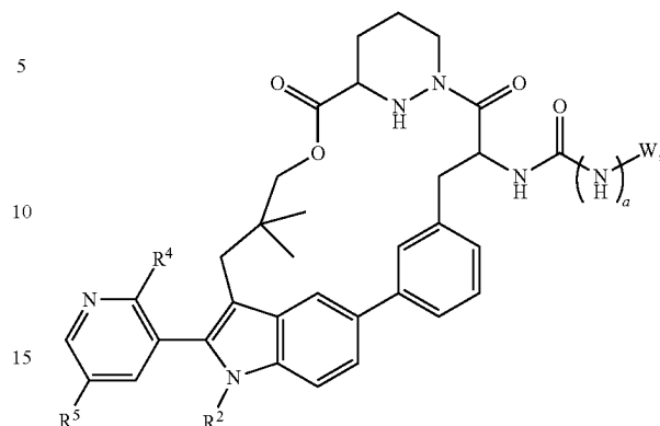
Formula IIIa-3
