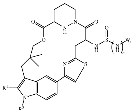
Formula VIIIa
