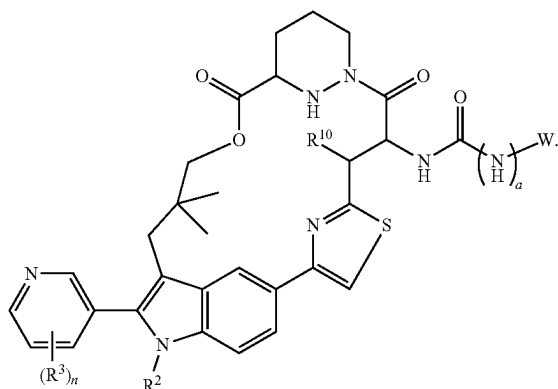
Formula IIb-2
