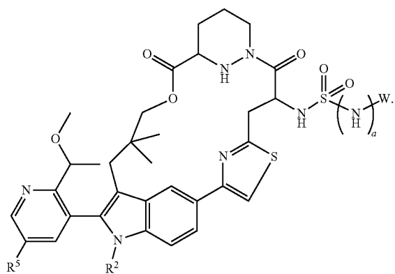
Formula Va-4
