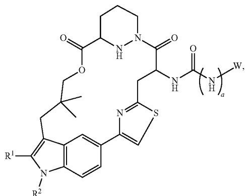
Formula IIa
