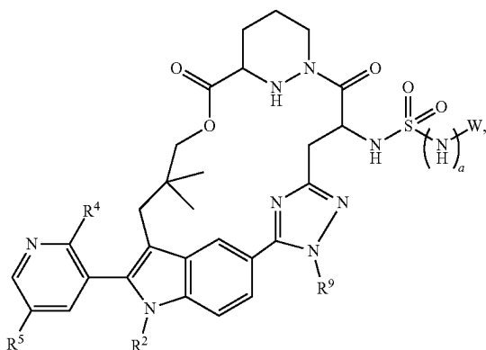
Formula VIIa-3
