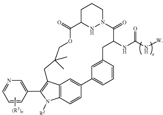
Formula IIIa-2
