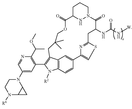
Formula IIa-7
