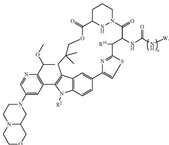
Formula IIb-9
