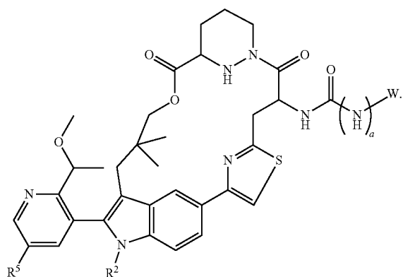
Formula IIa-4
