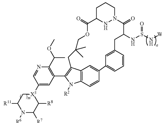
Formula IXa-5
