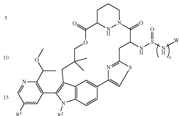
Formula VIIIa-4
