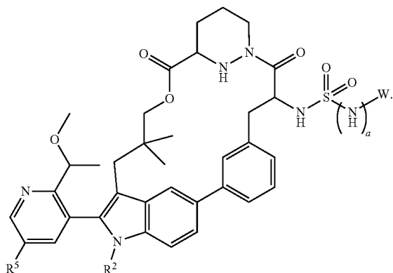
Formula VIa-4
