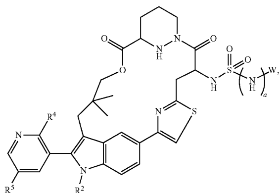
Formula Va-3
