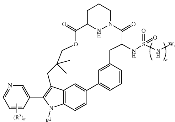
Formula VIa-2
