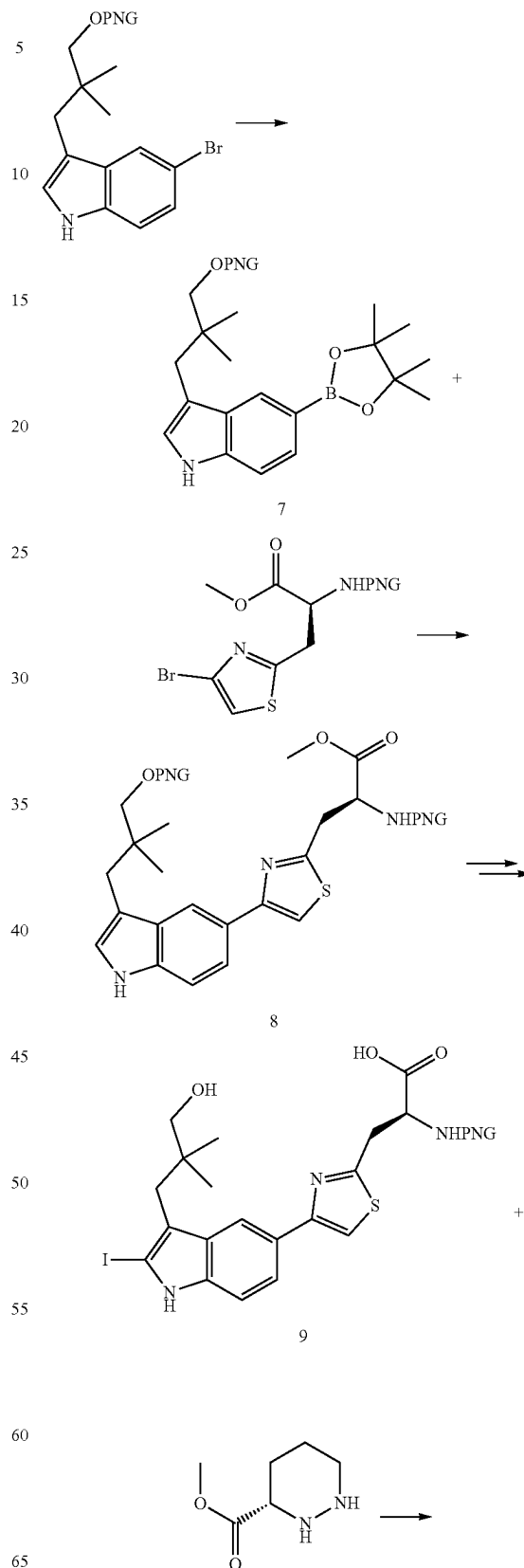
Scheme 2. Alternative general synthesis of macrocyclic esters
