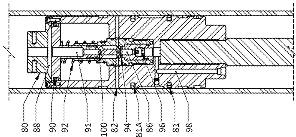
FIGURE 5B PLUNGER UNCOMPRESSED
