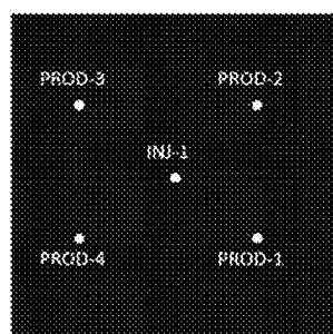
Five-spot well pattern
