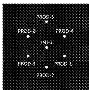
Inverted seven-spot well pattern
