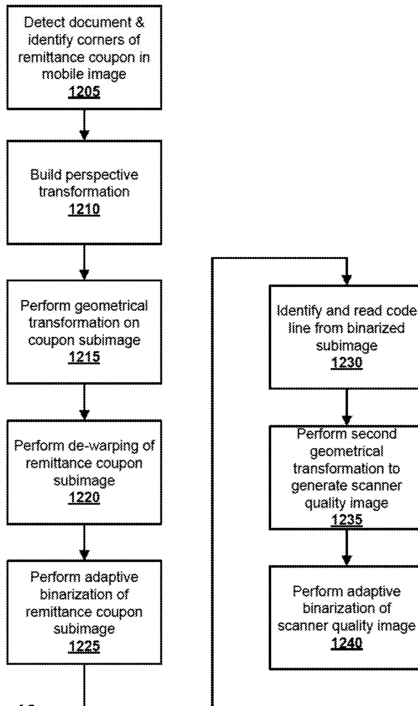
FIG. 12 Image Correction Module
