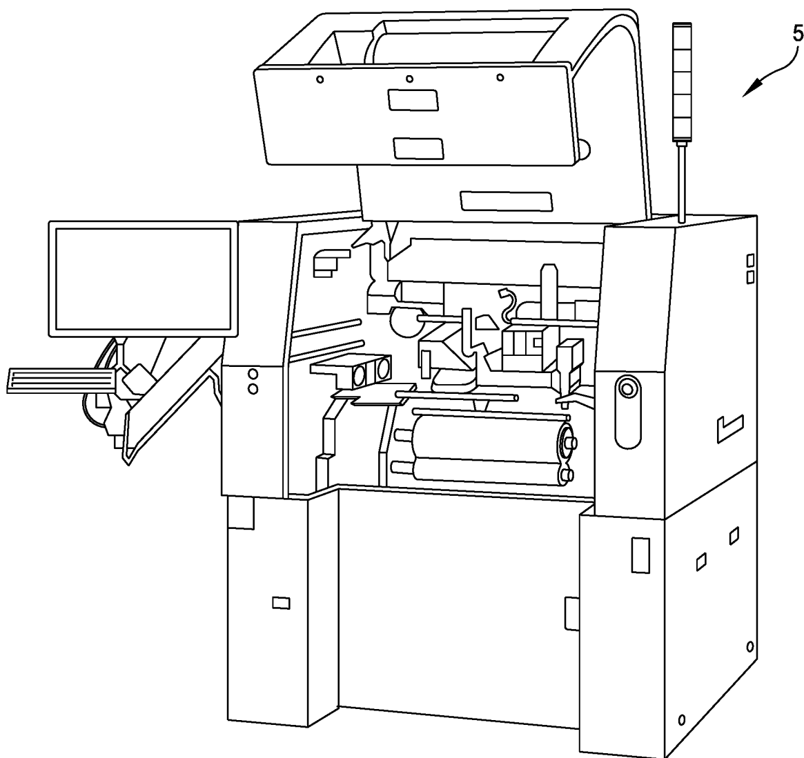
FIG. 1 (PRIOR ART)
