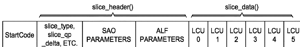
FIG. 5 (PRIOR ART)
