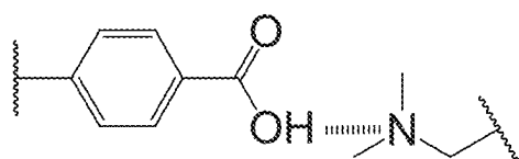
Carboxylic acid
