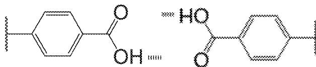
Carboxylic acid
