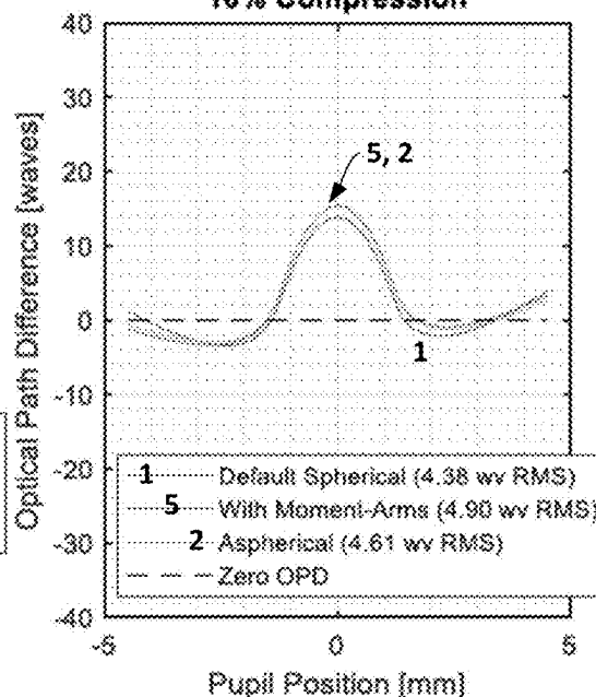
FIG. 11B OPD Maps for 10% Compression
