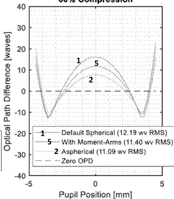
FIG. 11D OPD Maps for 60% Compression
