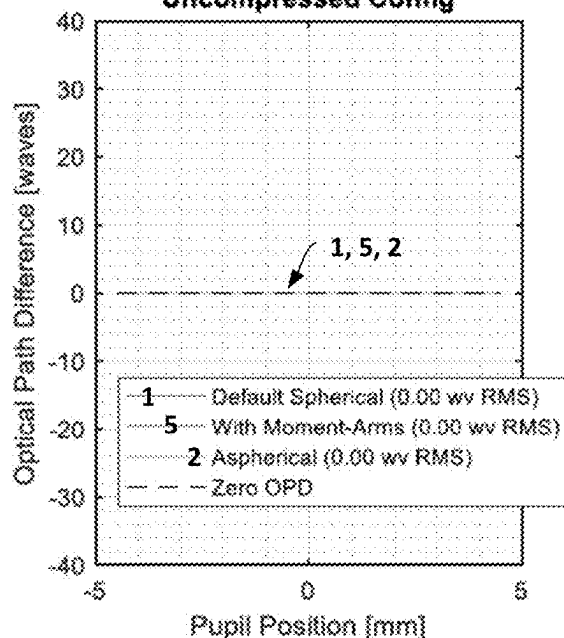
FIG. 11A OPD Maps for Uncompressed Config
