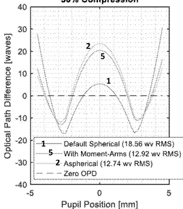
FIG. 11C OPD Maps for 30% Compression
